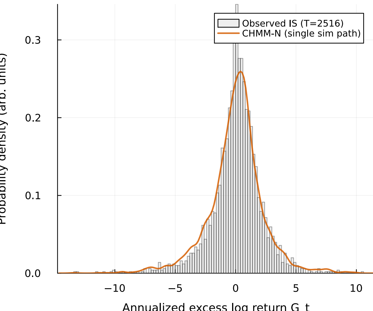
(a) IS return density | KS pass rate = 88.5% of 1000 paths at alpha=0.05
