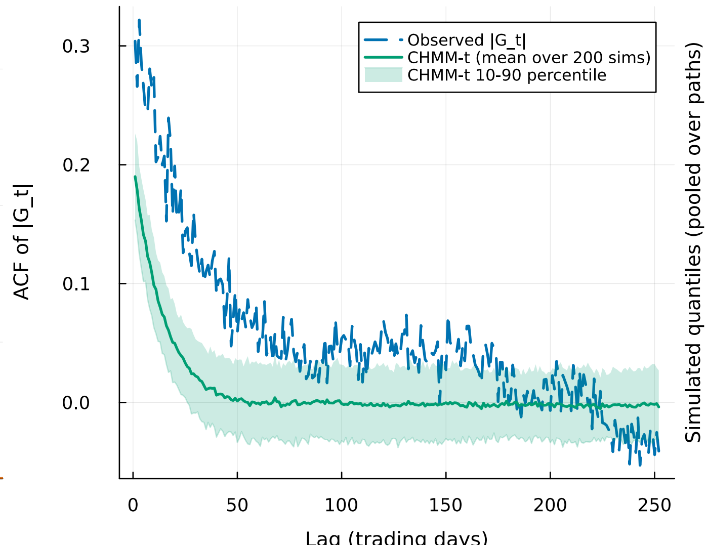
(b) ACF of |G_t| | lag 1..252 (trading days)
