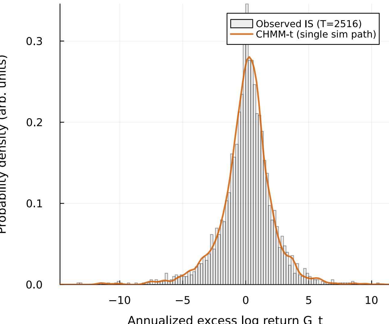
(a) IS return density | KS pass rate = 92.3% of 1000 paths at alpha=0.05
