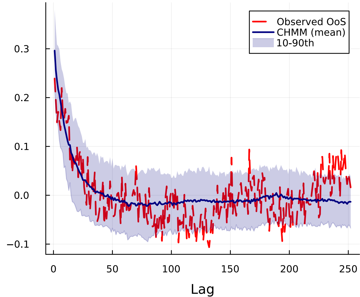
(c) OoS ACF( |G_t| )
