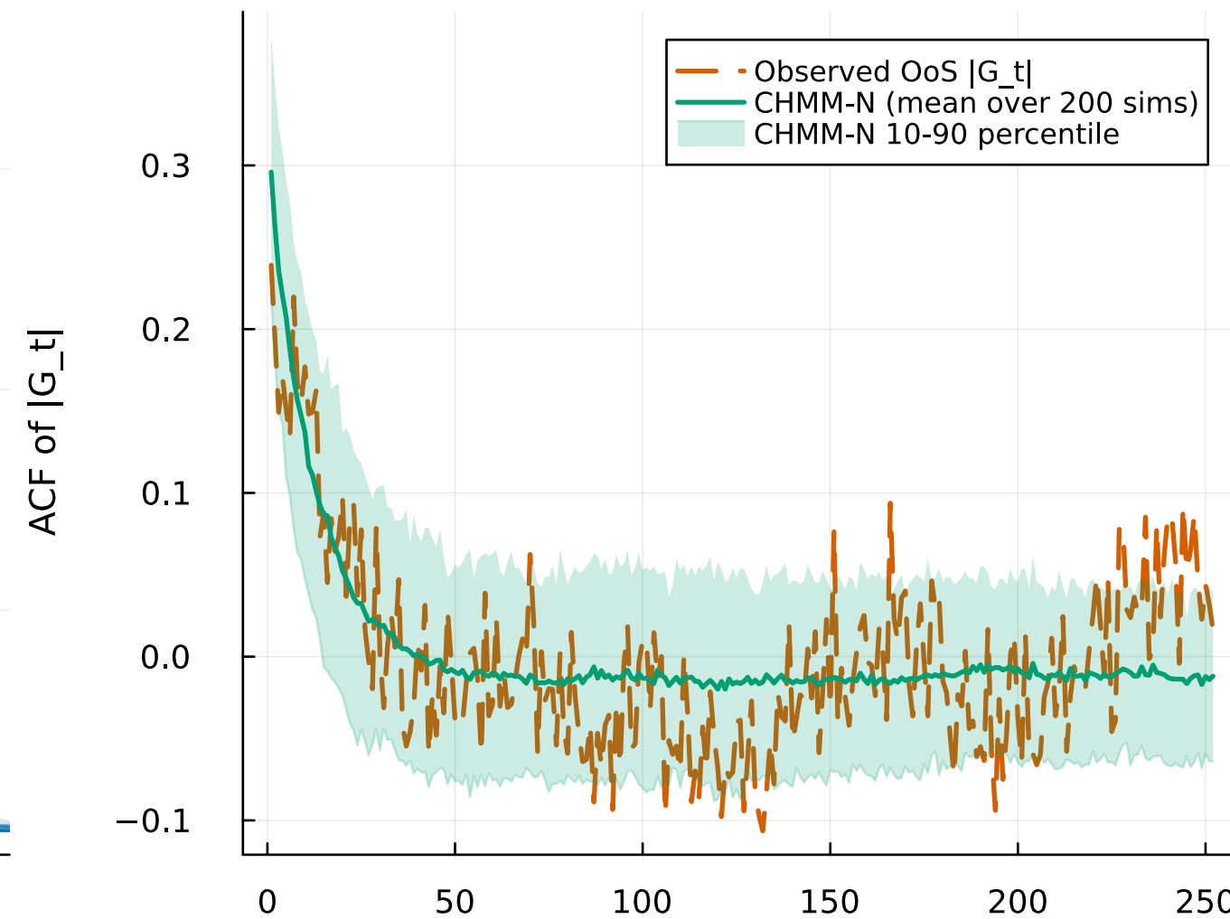
(c) OoS ACF of |G_t| | lag 1..252 (trading days)
