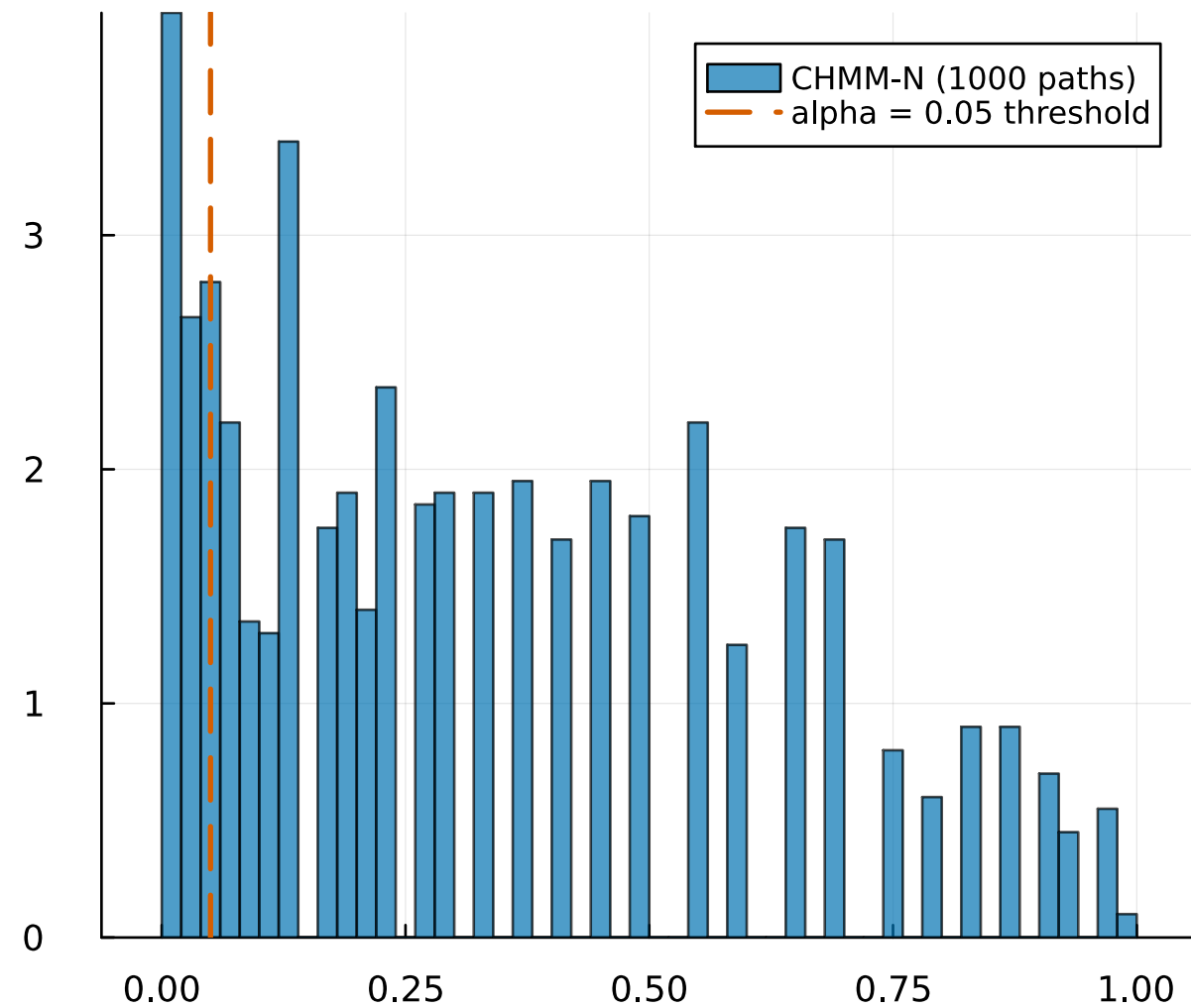
(a) OoS KS p-values | pass rate = 82.8% above \alpha=0.05
