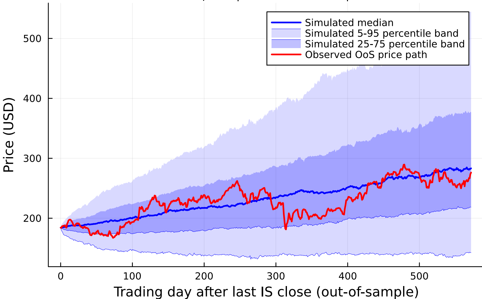
Pipeline A — AAPL OoS price fan | CHMM-L, K=18 500 simulated paths | S0 = last IS VWAP | dt = 1/252
