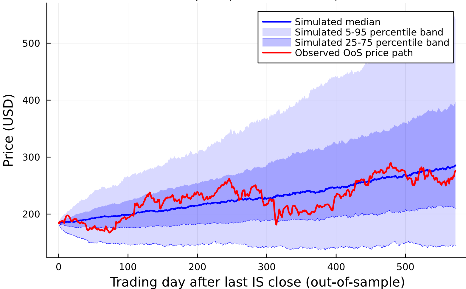
Pipeline A — AAPL OoS price fan | CHMM-t, K=18 500 simulated paths | S0 = last IS VWAP | dt = 1/252
