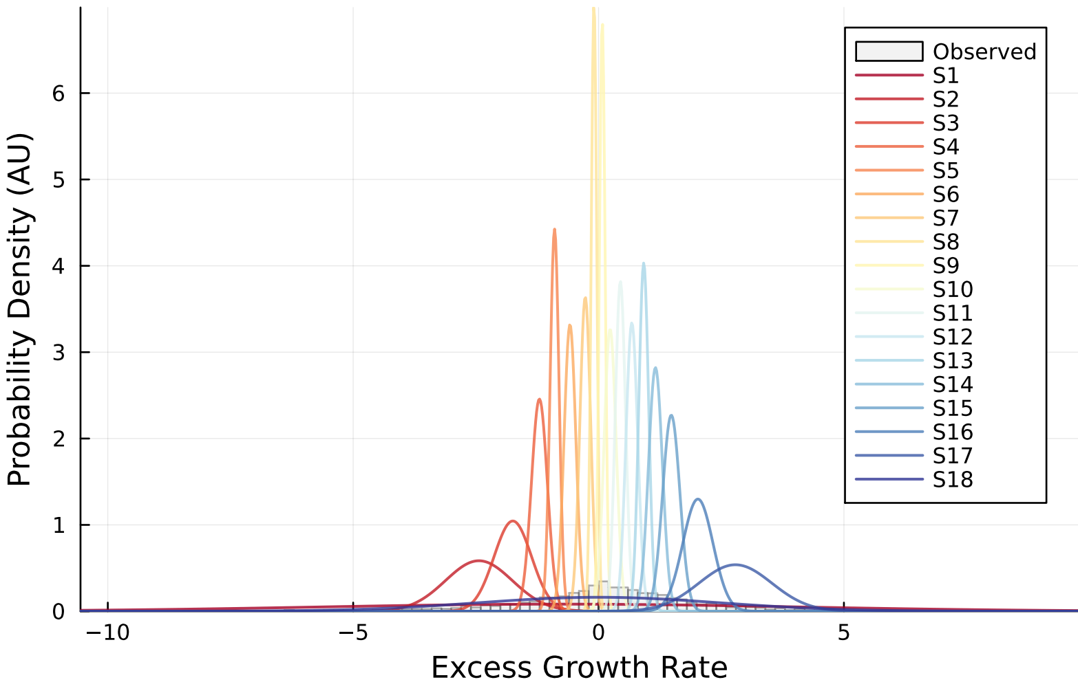
Emission Distributions (SPY, K=18)
