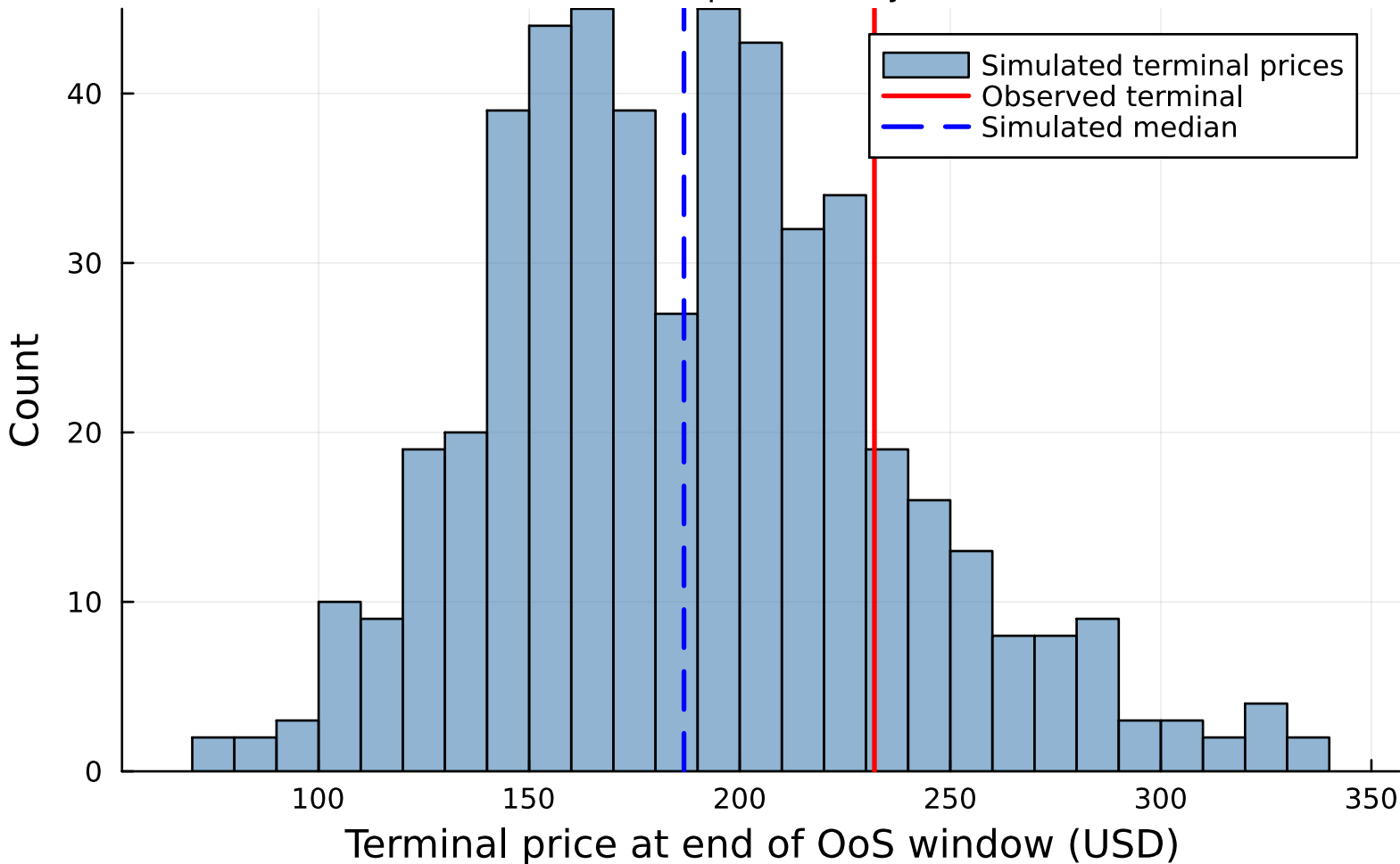
Pipeline A — JNJ terminal-price distribution | CHMM-N, K=18 500 simulated paths at day 572 OoS
