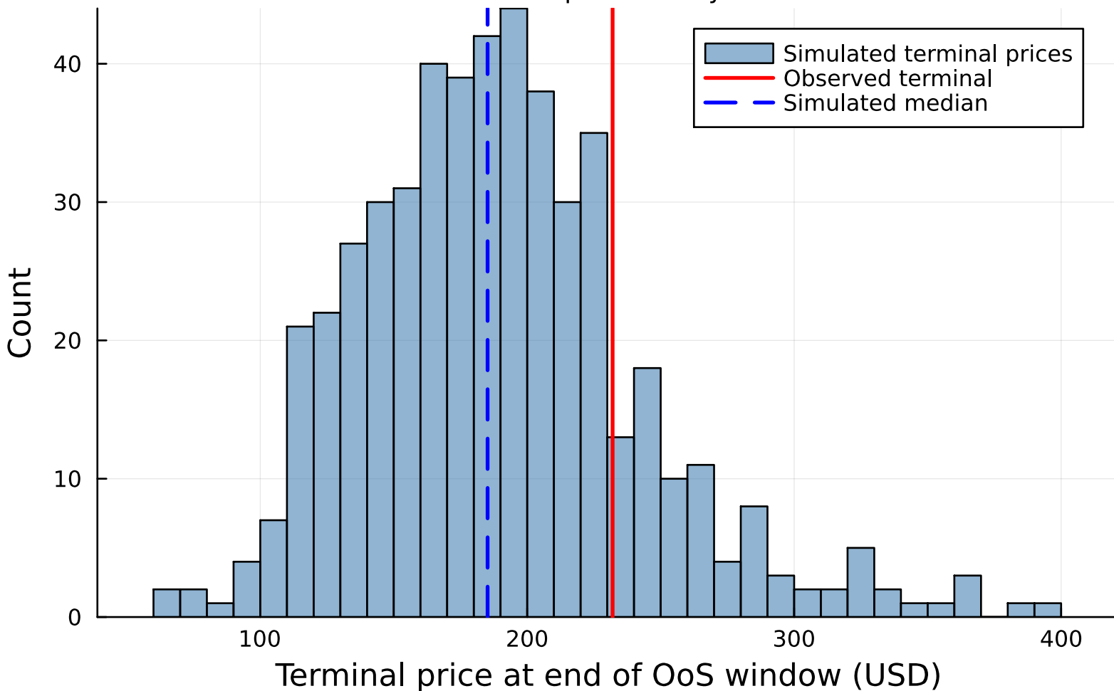
Pipeline A — JNJ terminal-price distribution | CHMM-t, K=18 500 simulated paths at day 572 OoS
