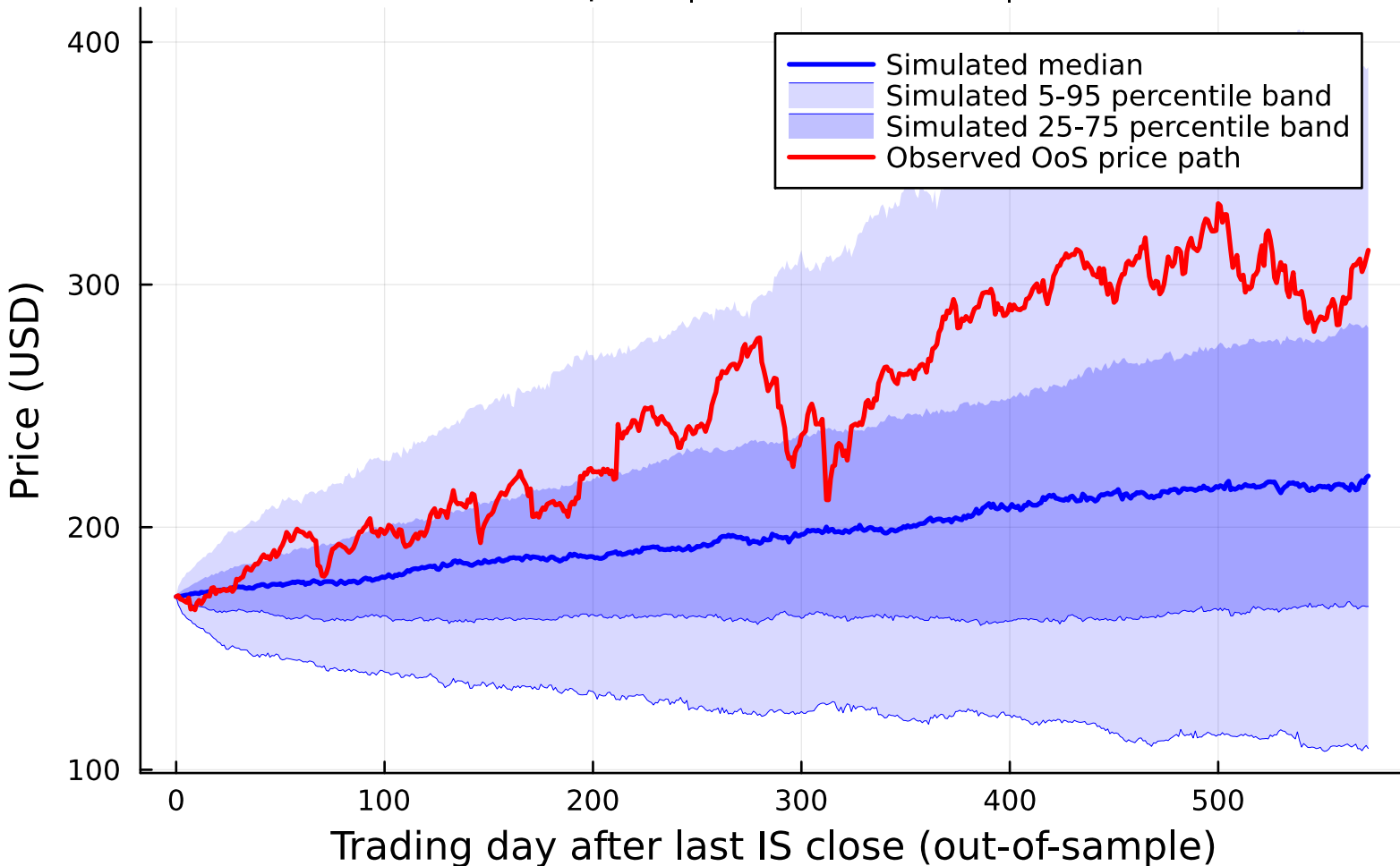
Pipeline A — JPM OoS price fan | CHMM-N, K=18 500 simulated paths | S0 = last IS VWAP | dt = 1/252
