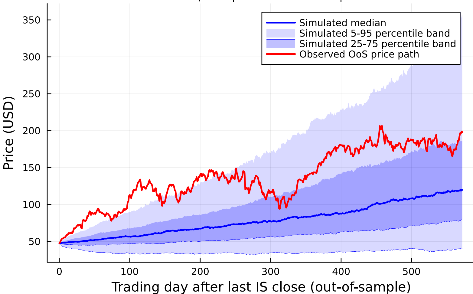
Pipeline A — NVDA OoS price fan | CHMM-L, K=18 500 simulated paths | S0 = last IS VWAP | dt = 1/252
