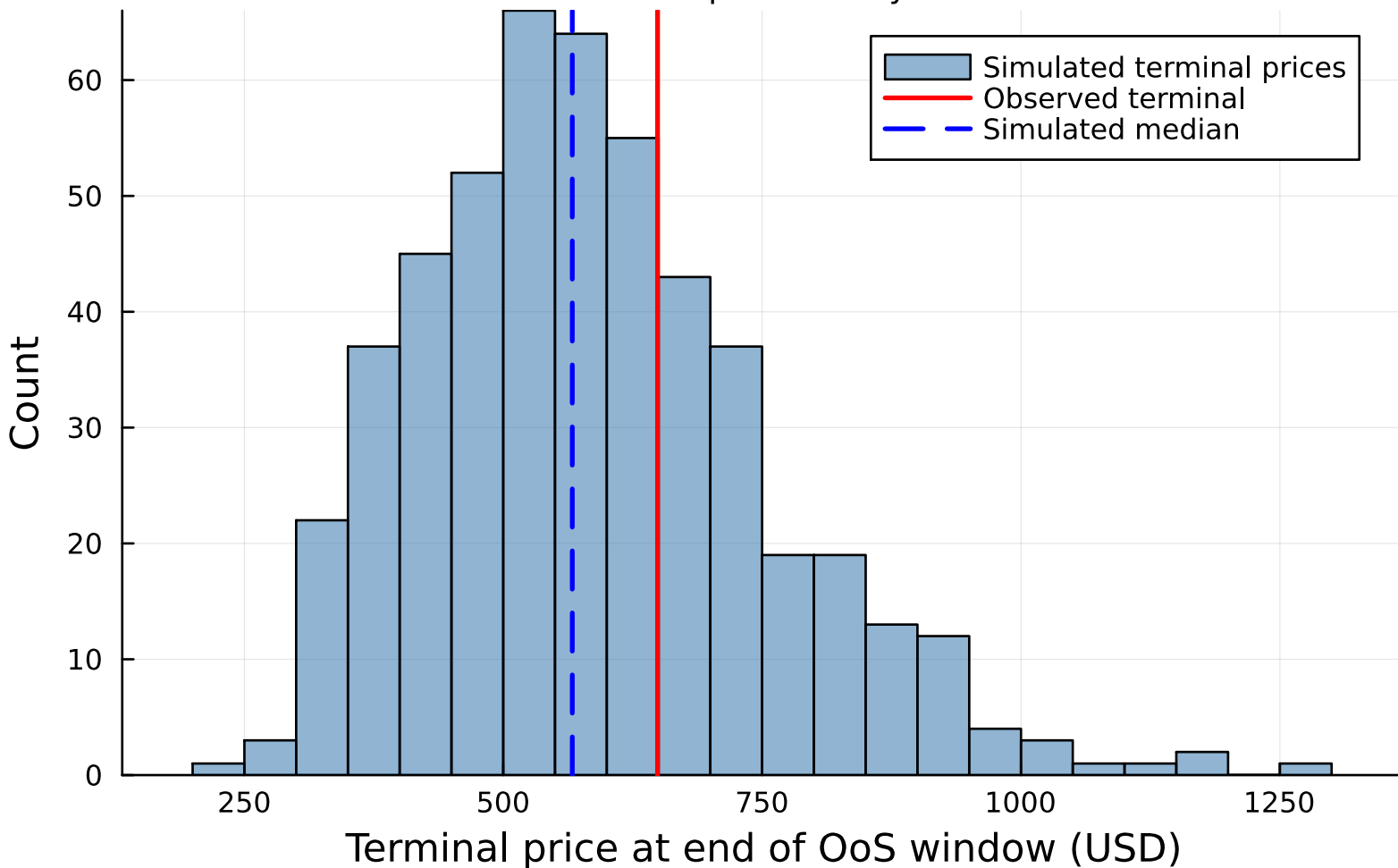
Pipeline A — QQQ terminal-price distribution | CHMM-t, K=18 500 simulated paths at day 572 OoS
