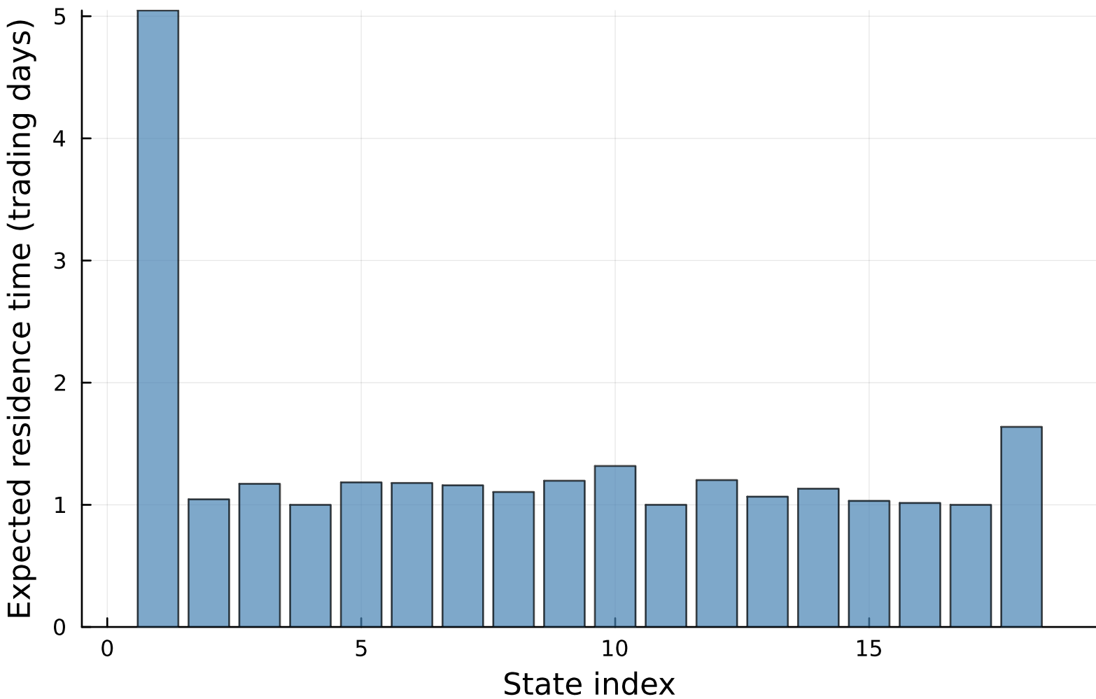
Natural residence time 1/(1 - T_{ii}) | SPY | CHMM-t, K=18
