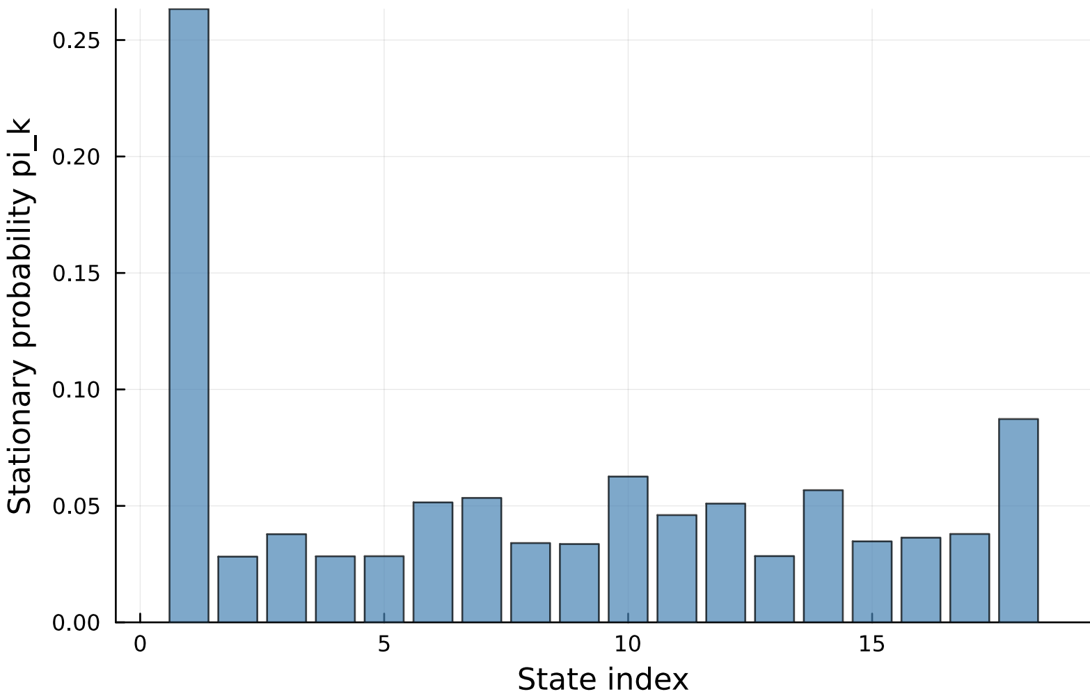
Stationary distribution \pi (= left eigenvector of T ) | SPY | CHMM-t, K=18
