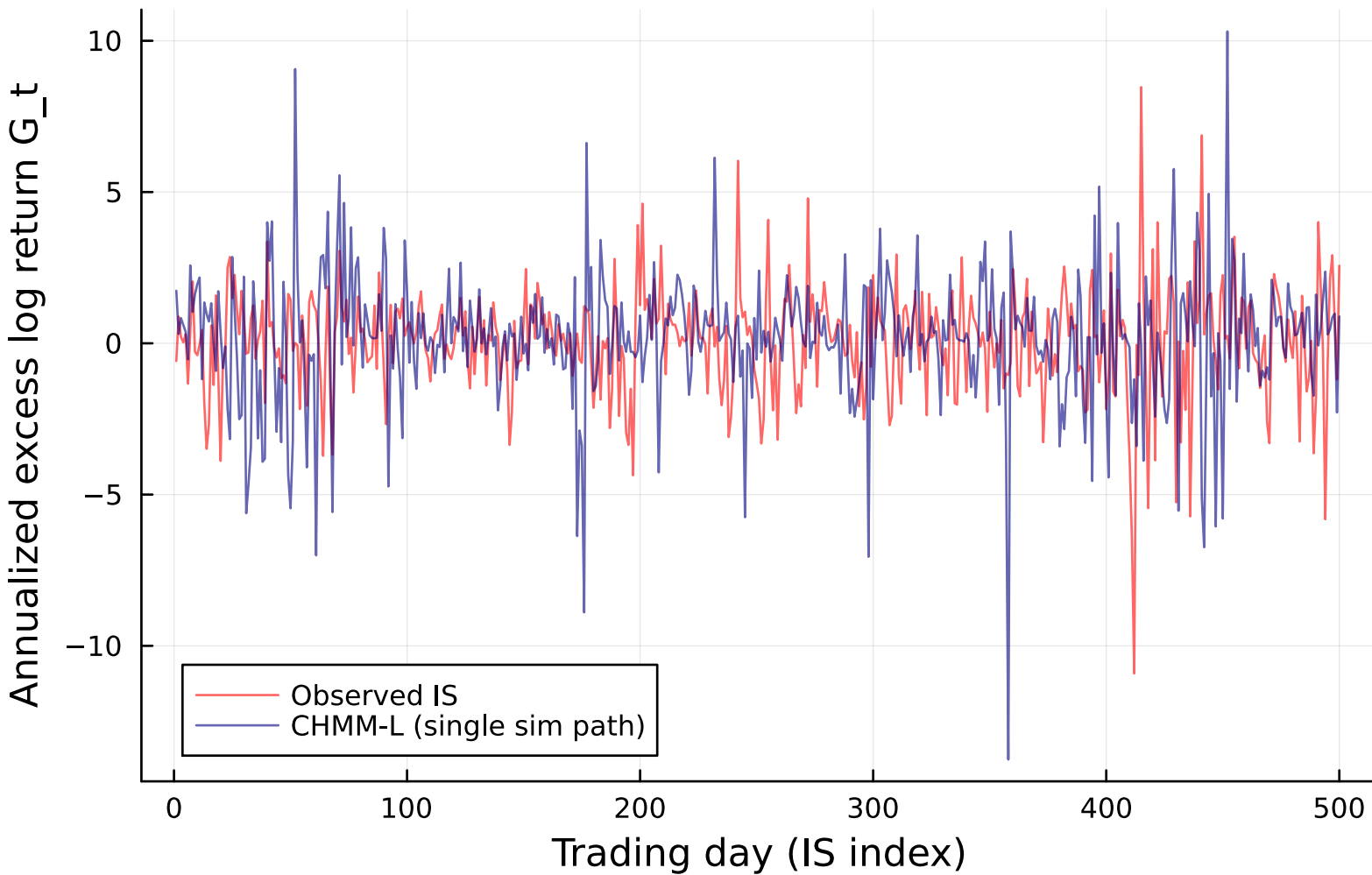
Sample return trajectory (first 500 IS days) | SPY | CHMM-L, K=18
