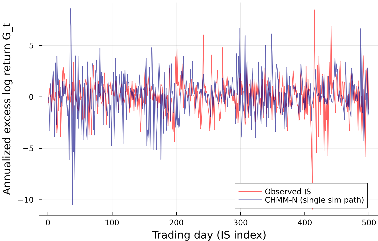
Sample return trajectory (first 500 IS days) | SPY | CHMM-N, K=18
