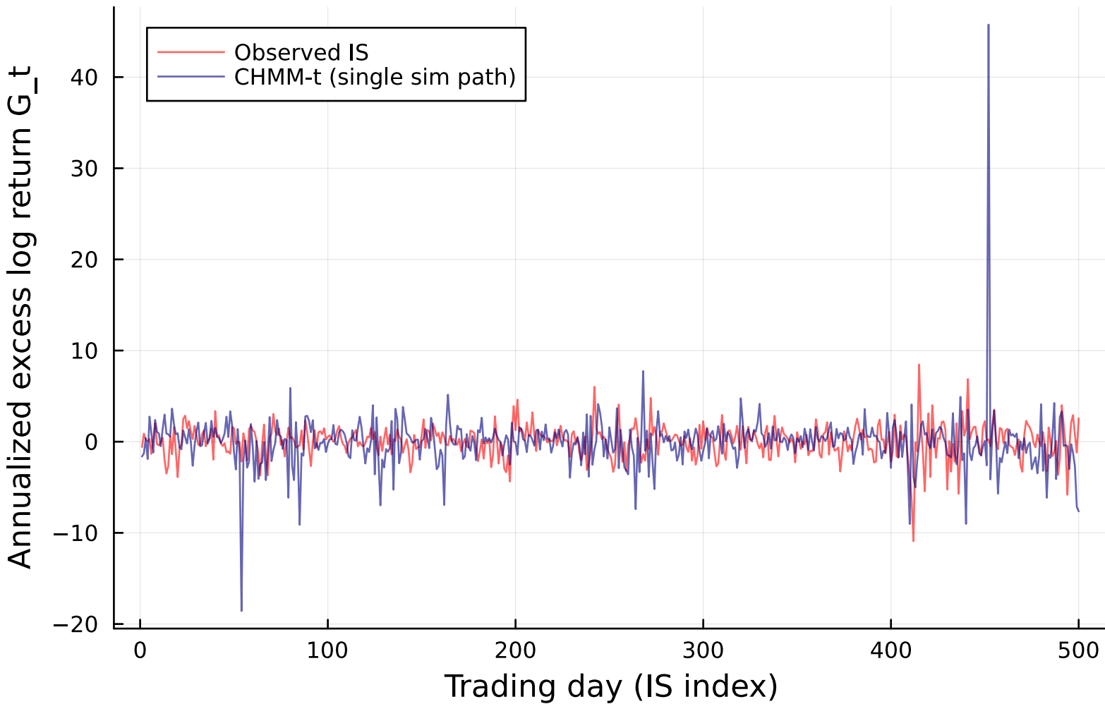
Sample return trajectory (first 500 IS days) | SPY | CHMM-t, K=18
