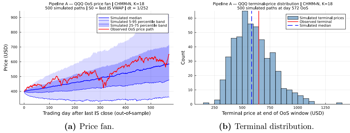
Figure 34. QQQ OoS price fan and terminal distribution, CHMM-N (Pipeline A, K = 18 , 500 simulated paths, T_{\text{OoS}} = 572 ; plotting conventions as above).
