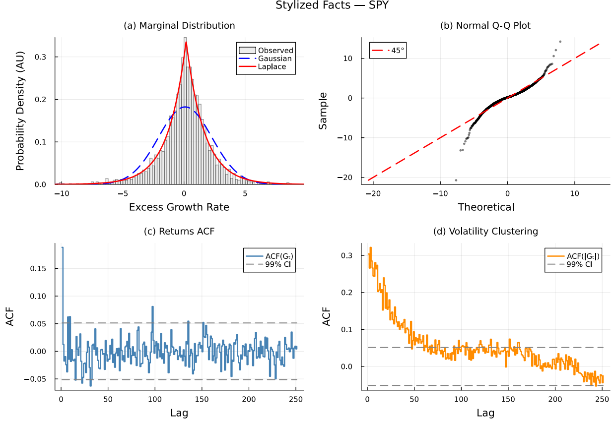
Figure 7. Empirical stylized facts of SPY daily excess growth rates (IS, 2014-01-03 through 2024-01-03). Panel (a): leptokurtic marginal distribution with Gaussian and Laplace fits. Panel (b): normal Q-Q plot confirming heavy tails. Panel (c): near-zero autocorrelation of raw returns. Panel (d): persistent autocorrelation of absolute returns characterizing volatility clustering.
