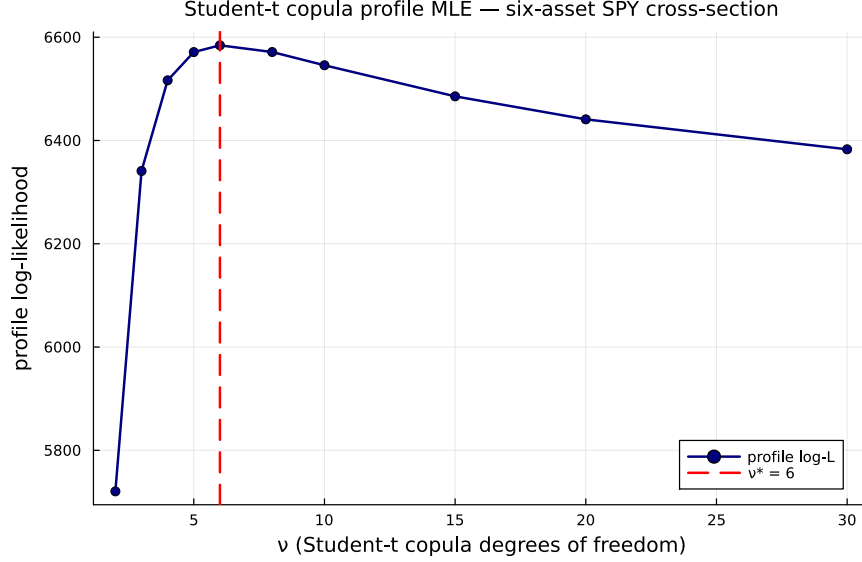
Figure 35. Profile log-likelihood of the Student-t copula used inside Pipeline B on the six-asset SPY cross-section (SPY, NVDA, JNJ, JPM, AAPL, QQQ; IS window 2014-01-03 through 2024-01-03). The vertical axis is the profile log-likelihood evaluated at each degrees-of-freedom value \nu on the grid \{2, 3, 4, 5, 6, 8, 10, 15, 20, 30\} ; the dashed red line marks the profile MLE \nu^* = 6 (peak value 6157.47). The CHMM-N marginals are held fixed at the Pipeline A per-asset fits while \nu is varied.
