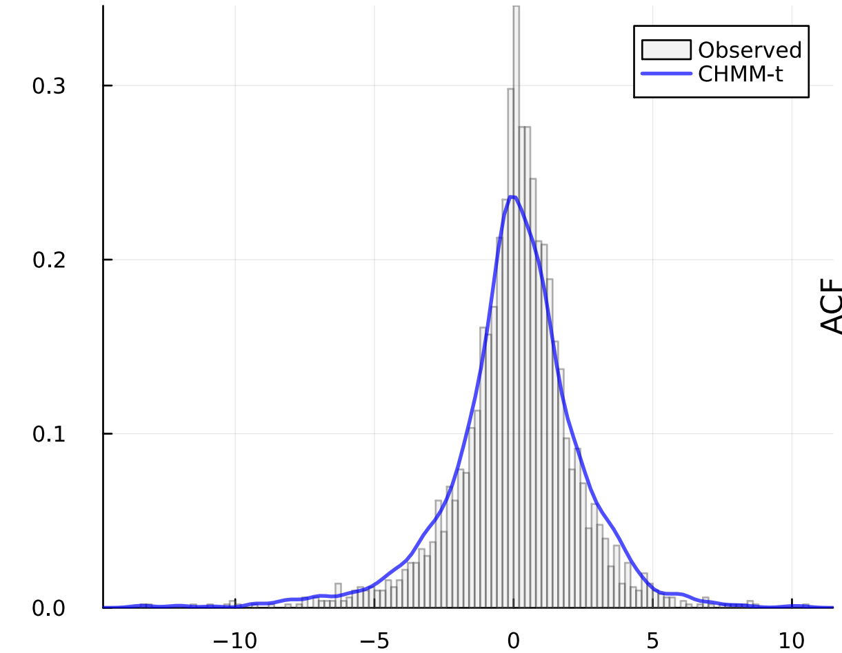
(a) IS Density (KS: 91.1%)
