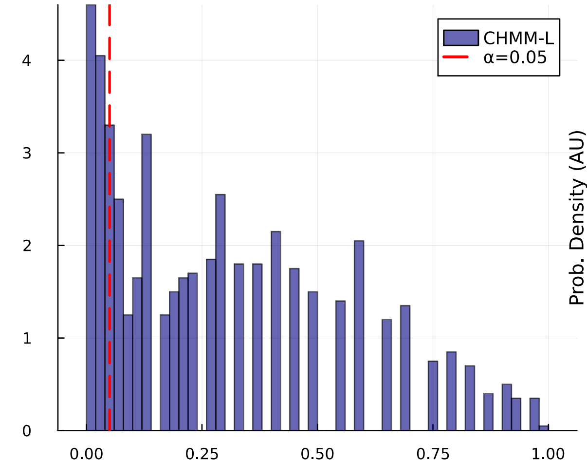
(a) OoS KS p-values (pass: 77.9%)
