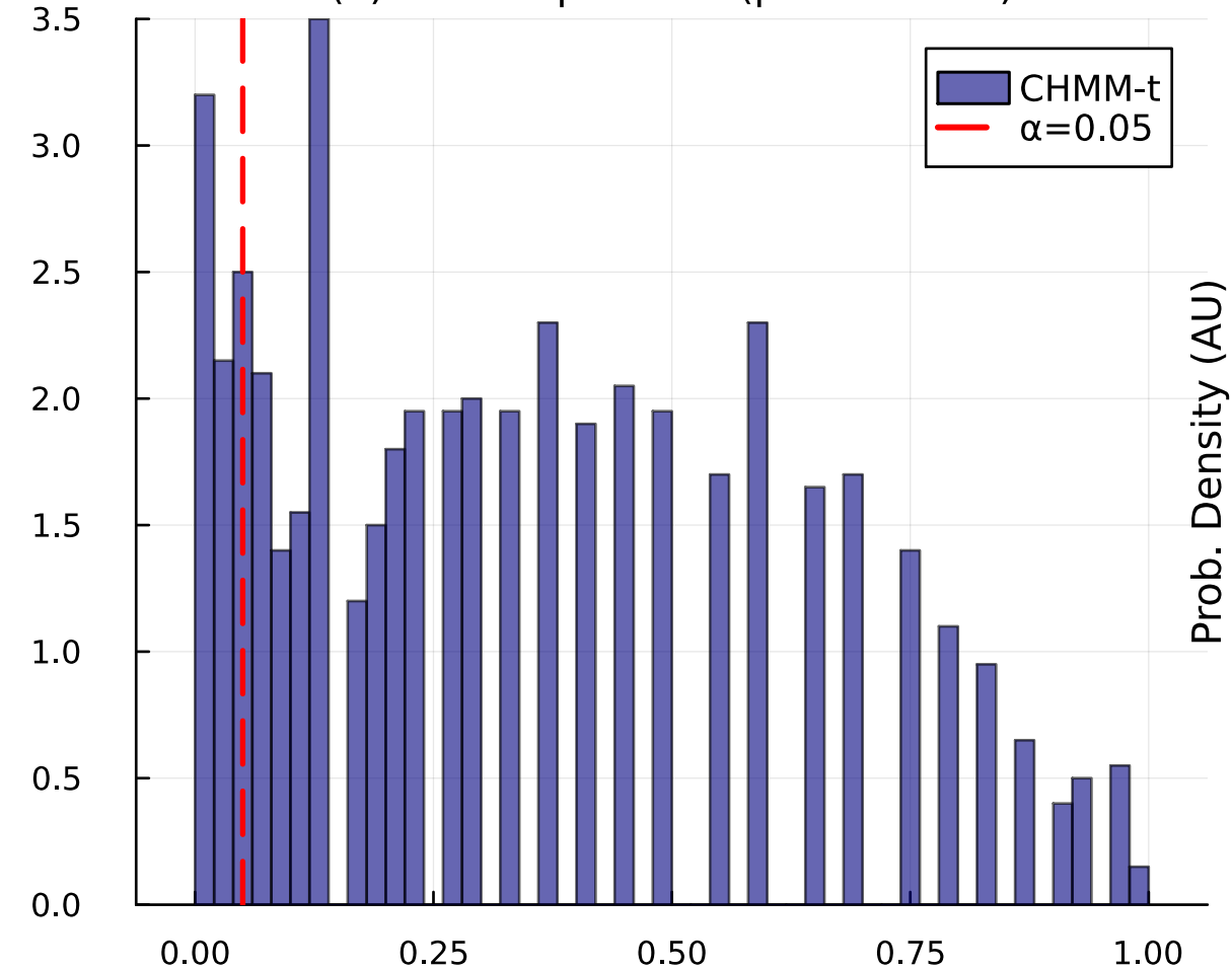
(a) OoS KS p-values (pass: 86.2%)
