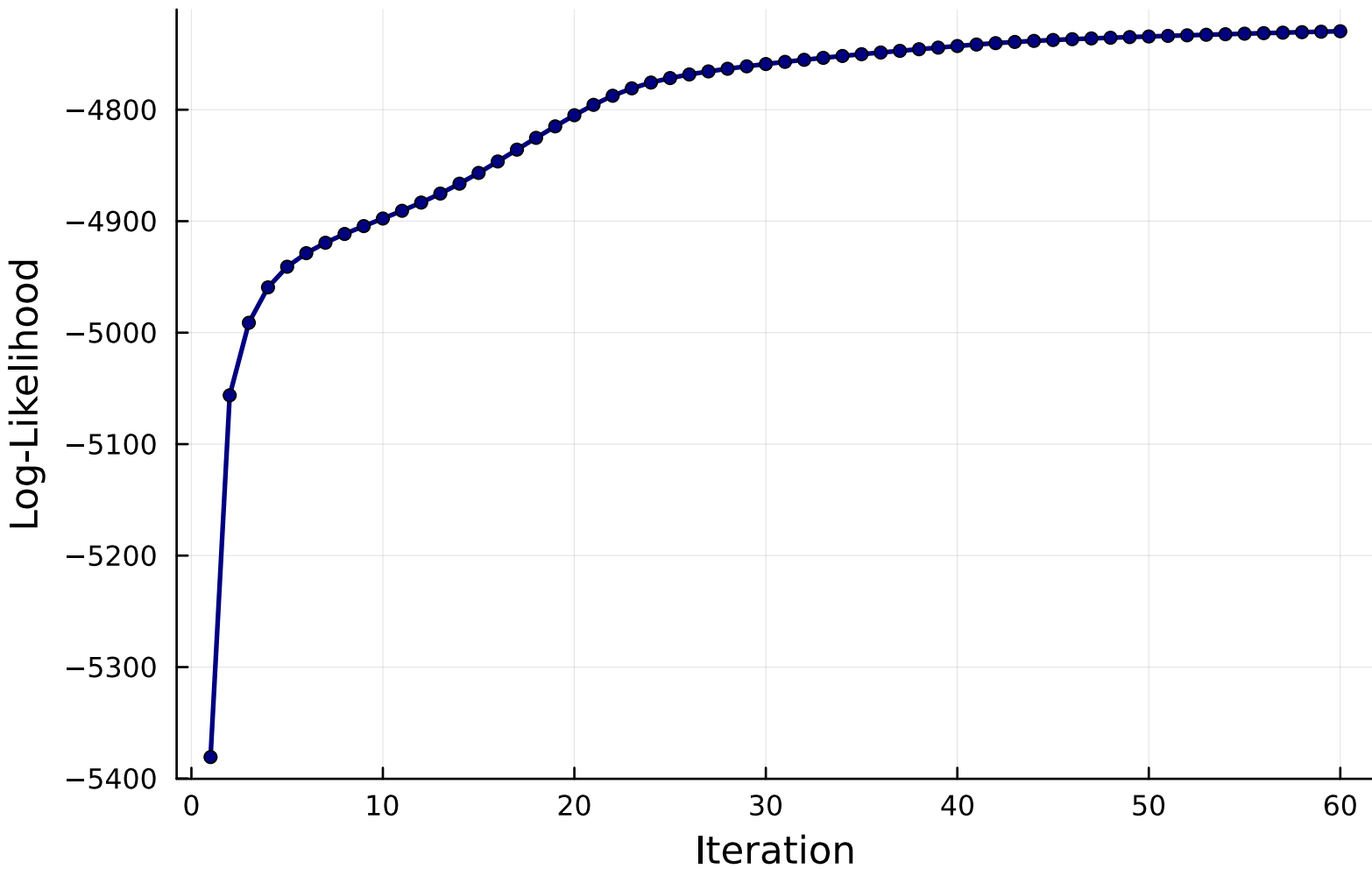
Convergence (CHMM-t, K=18)
