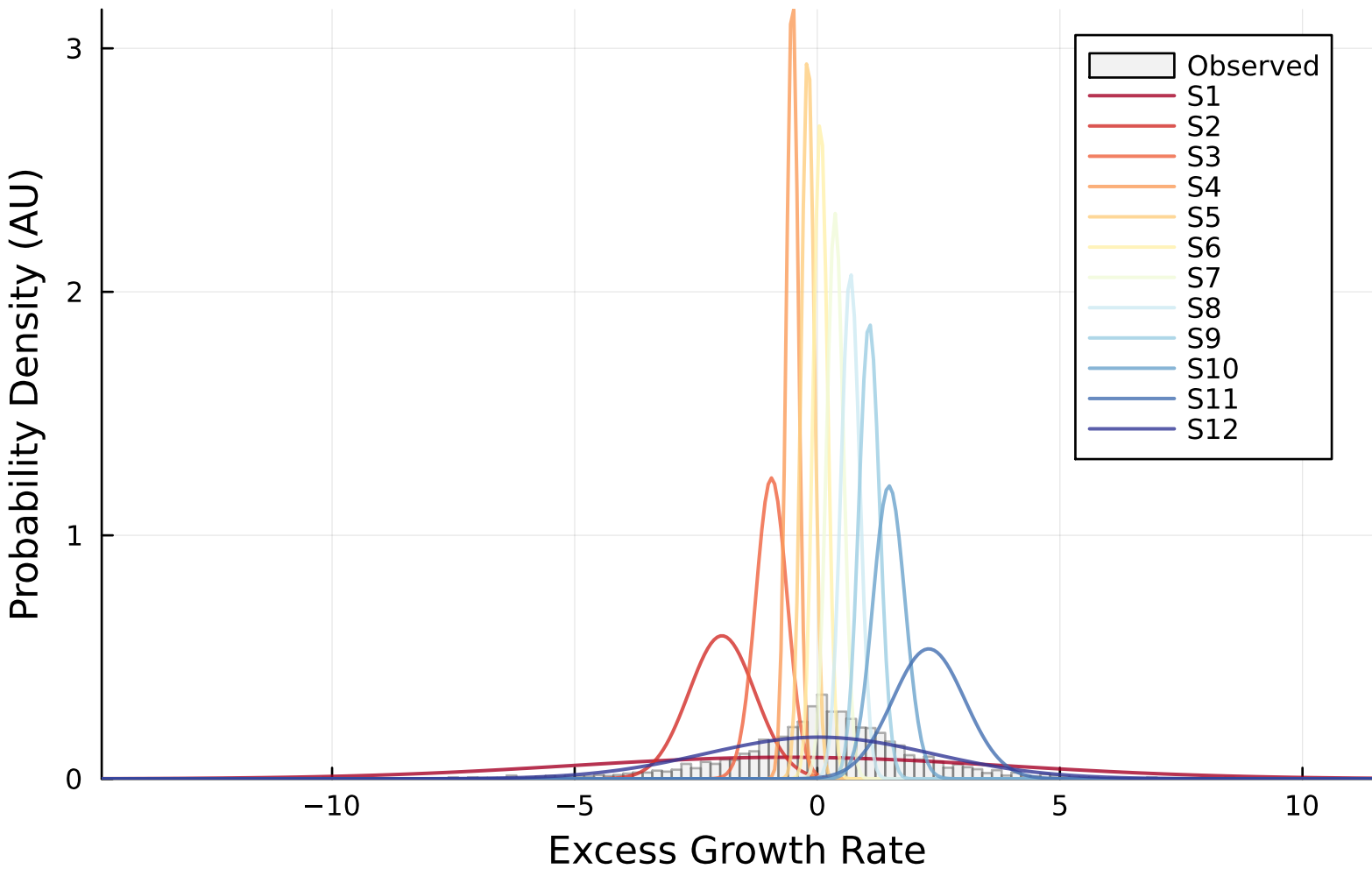
Emission Distributions (CHMM-N, K=12)
