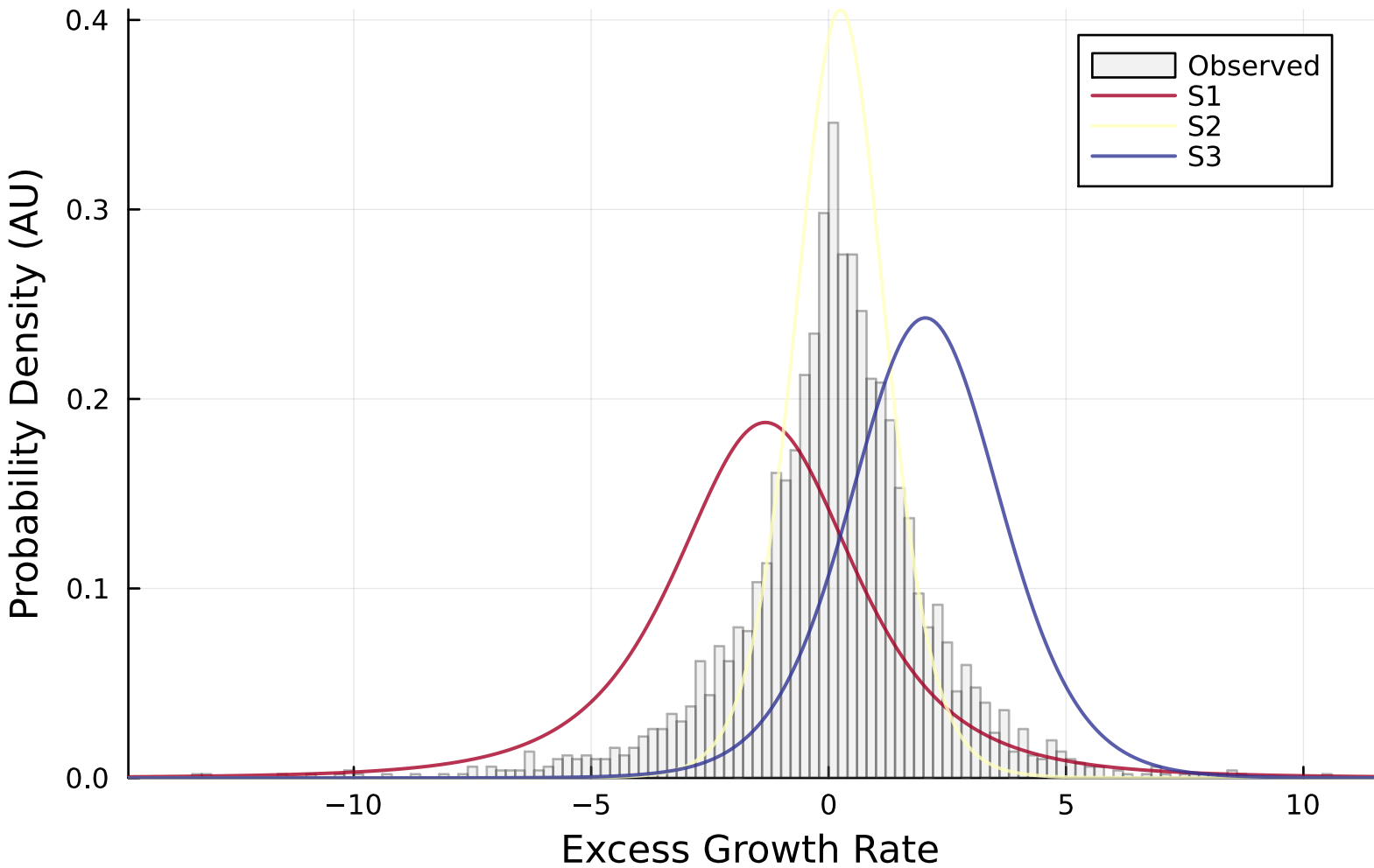
Emission Distributions (CHMM-t, K=3)
