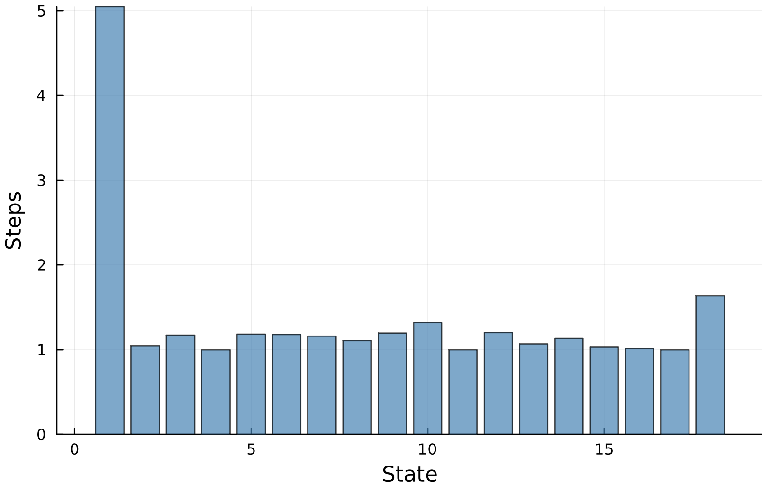
Natural Residence Times (CHMM-t, K=18)
