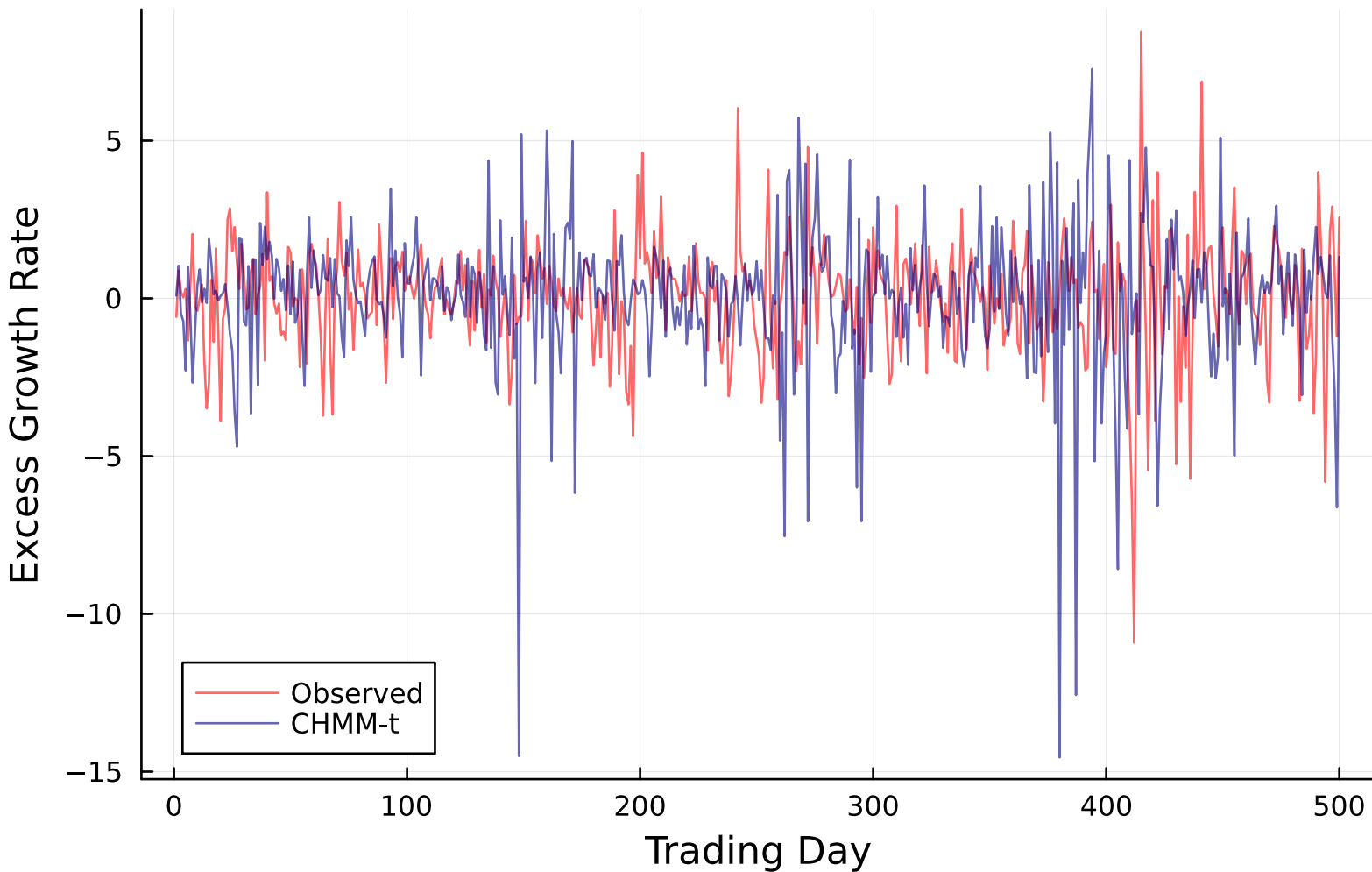
Return Trajectory (CHMM-t, K=18)
