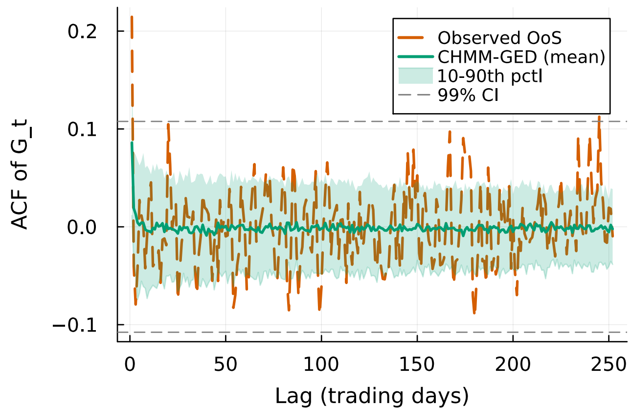
OoS ACF of G_t (raw returns)
