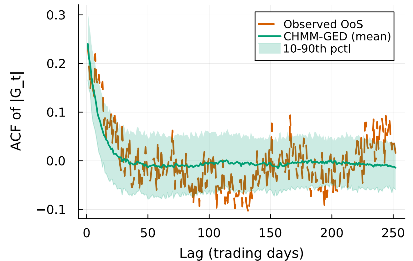
OoS ACF of |G_t|
