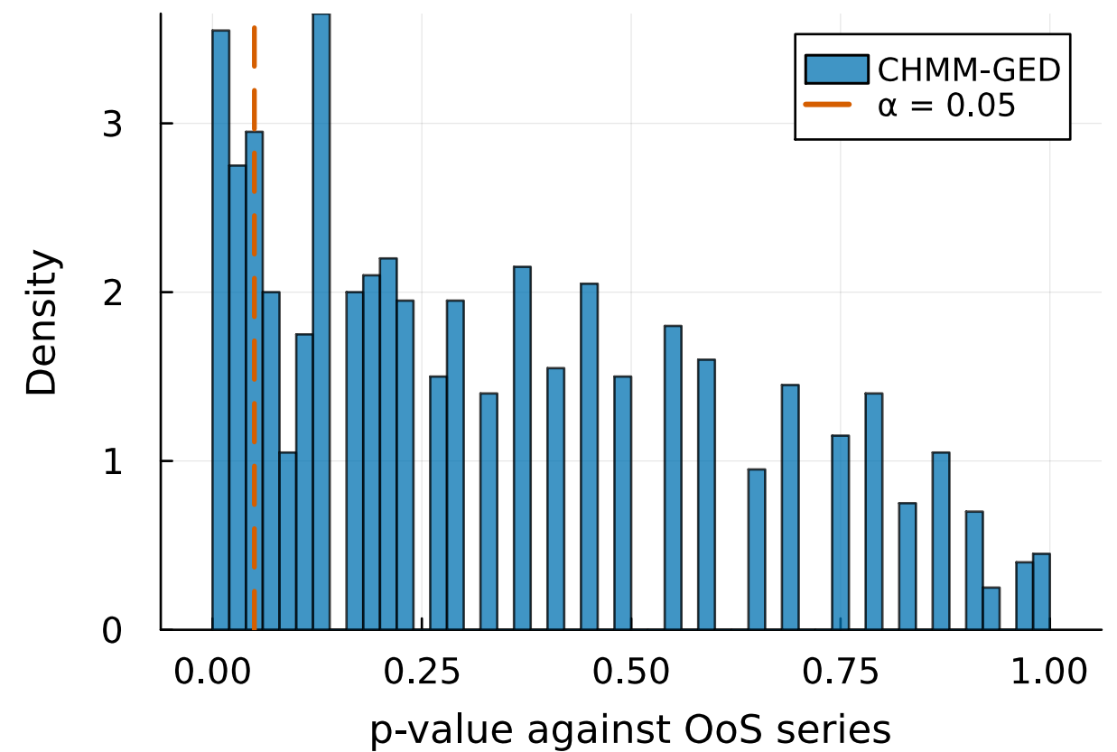
OoS KS p-values (pass: 83.8%)
