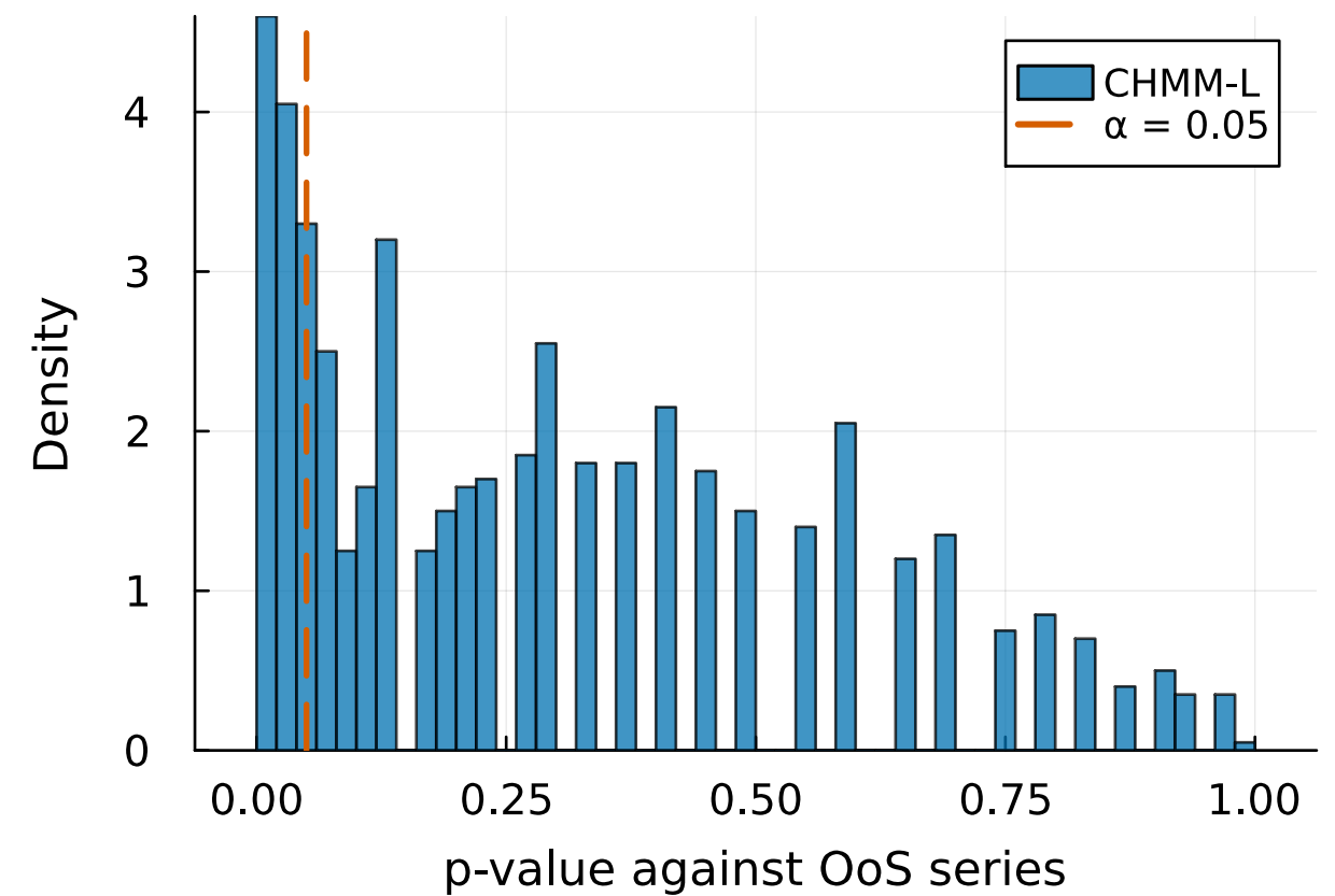
OoS KS p-values (pass: 77.9%)
