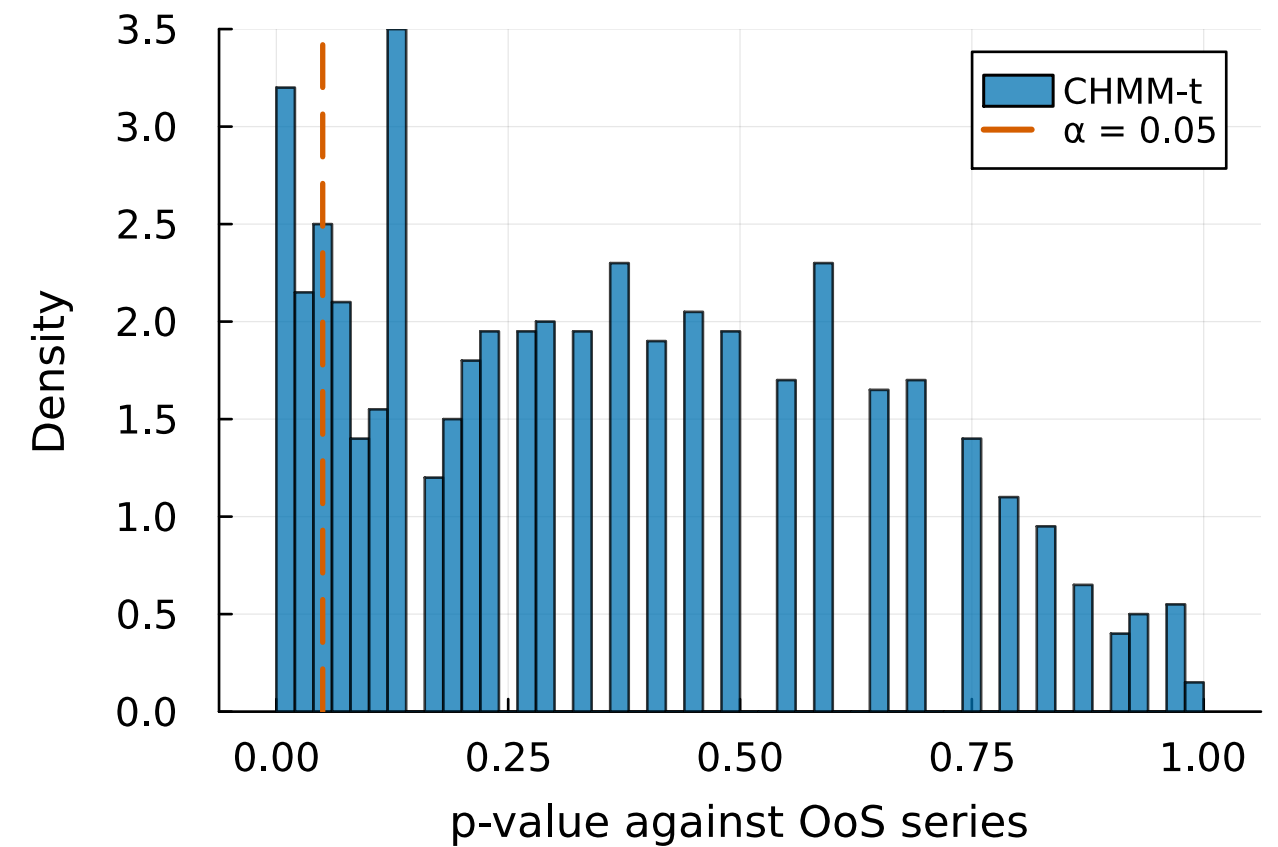
OoS KS p-values (pass: 86.2%)
