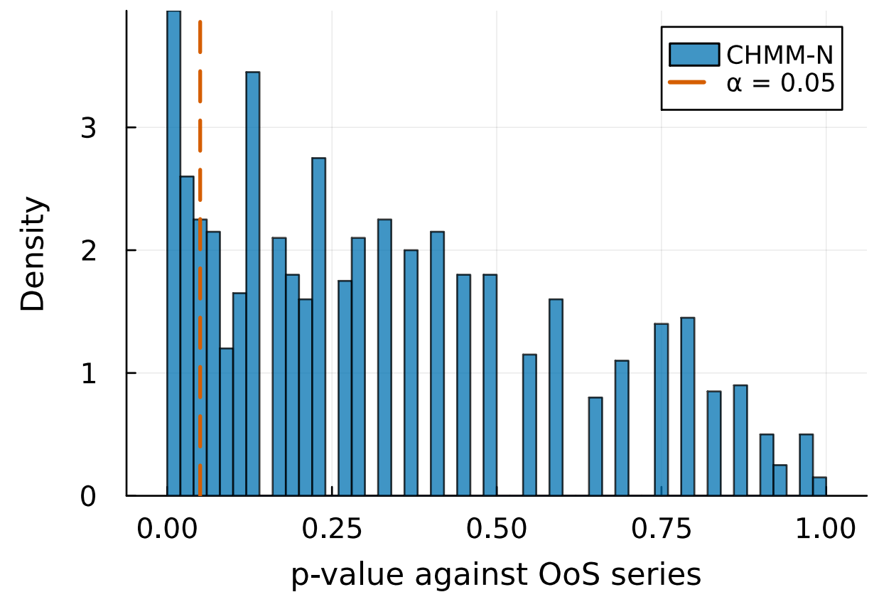
OoS KS p-values (pass: 84.2%)
