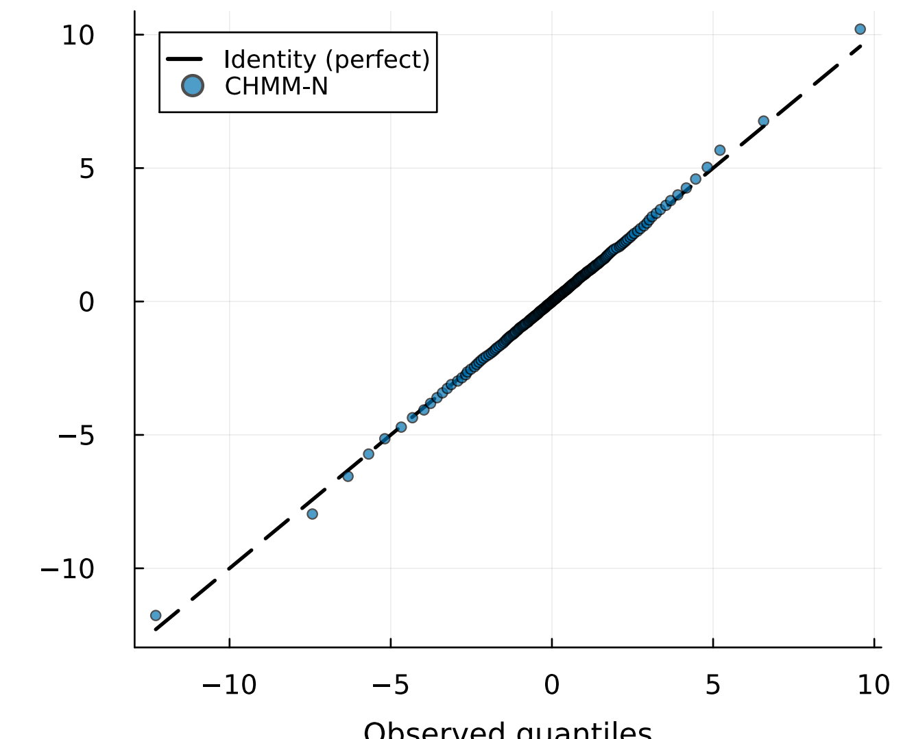
(c) Tail Q-Q plot (0.1st-99.9th)
