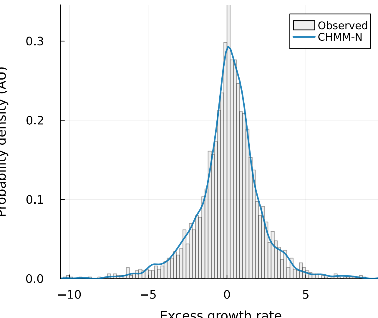
(a) IS density (KS: 94.1%)
