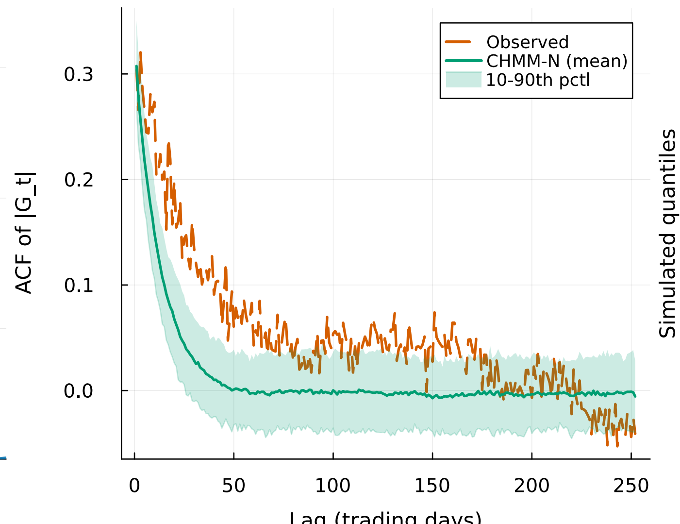
(b) ACF of |G_t|
