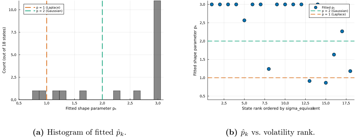
Figure 8. CHMM-GED per-state shape \hat{p}_k partition ( K = 18 , SPY IS, seed 20260420). The bimodal partition is visible at the upper bracket p_k = 3.0 and around the Laplace shape; the Laplace-shape cluster sits at the high-volatility ranks.
