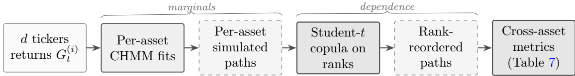
Figure 3. Schematic of Pipeline A (single-asset) and Pipeline B (cross-asset). Pipeline A fits a CHMM per ticker independently. Pipeline B reuses the per-asset fits as marginals and injects cross-asset dependence through a rank-based Student- t copula. The single-asset scaffold is shared across both pipelines.
