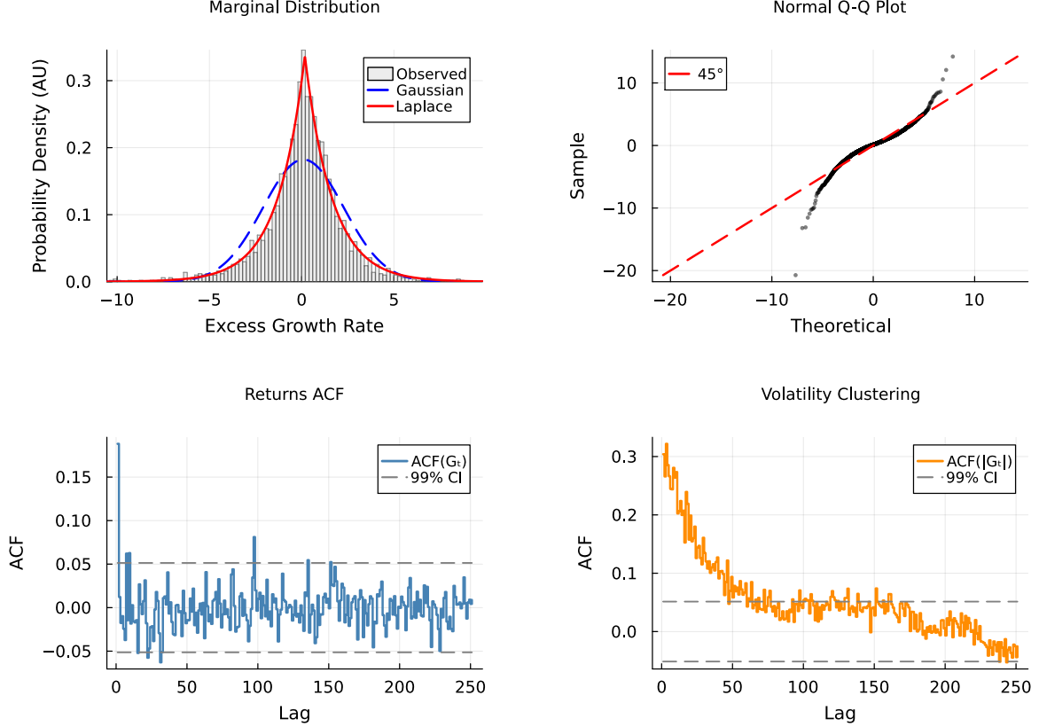
Figure 3. The three Cont stylized facts on SPY IS. Panel (a): empirical IS marginal density of the annualised excess log return G_t with maximum-likelihood Gaussian (blue dashed) and Laplace (red) overlays; Laplace tracks the central peak and tails decisively better. Panel (b): normal Q-Q plot showing the heavy-tailed deviation from the 45^\circ reference. Panel (c): empirical ACF of raw G_t at lags 1–252, with the 99% Bartlett confidence band (dashed grey); only lag 1 exits the band (microstructure noise), lags 2–252 sit inside, confirming negligible linear autocorrelation. Panel (d): empirical ACF of |G_t| on the same window, with the same 99% band; the slow decay over many lags is the volatility-clustering signature that motivates the spectral identity (8).
