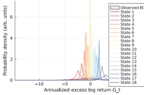
(c) CHMM-L (Laplace)
