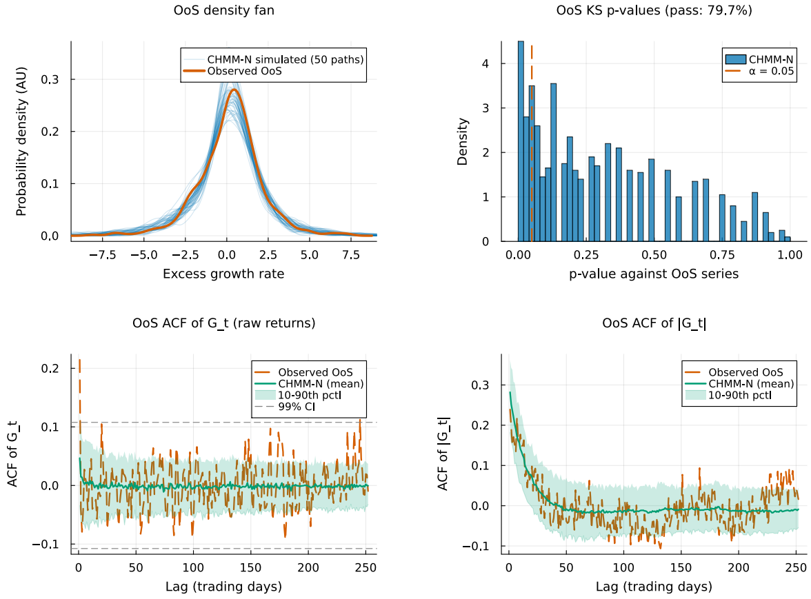
Figure 15. OoS SPY CHMM-N validation at K = 6 (Pipeline A, 1,000 simulated paths; panels as in Figure 5).
