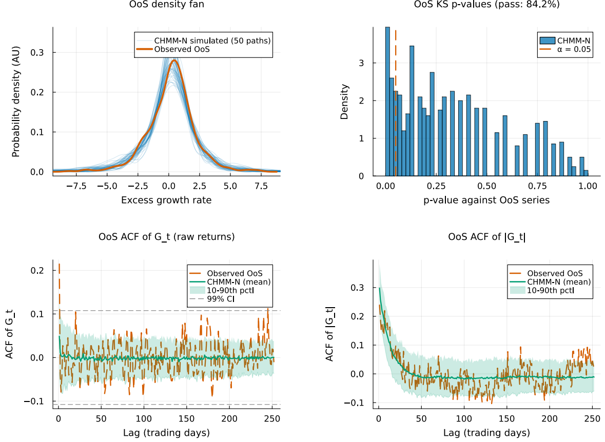
Figure 5. OoS CHMM-N validation on SPY ( K = 18 , 1,000 paths, T_{\text{OoS}} = 572 ). Panel (a): OoS return-density fan; blue thin curves = simulated densities, orange thick curve = observed OoS density. Panel (b): histogram of the 1,000 OoS KS p -values against the observed OoS series with the \alpha = 0.05 threshold (orange dashed). Panel (c): ACF of raw G_t on the OoS window (linear autocorrelation); orange dashed = observed, green = mean across sim paths, shaded band = 10th–90th percentile, dashed grey = 99% Bartlett band (wider than IS because T_{\text{OoS}} is shorter). Panel (d): ACF of |G_t| on the OoS window (volatility clustering); same colour conventions. The 2x2 layout parallels the IS comparison Figure 4.
