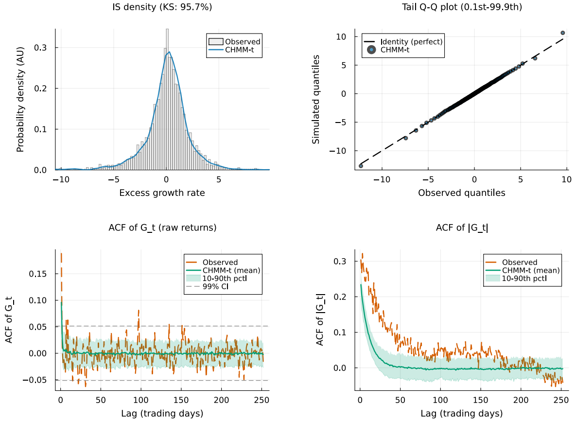
Figure 20. IS SPY model comparison at K = 18 for CHMM-t Student-t emissions (Pipeline A, 1,000 simulated paths). Panels show (a) marginal density with KS pass rate, (b) ACF of |G_t| , and (c) tail Q-Q plot. The CHMM-N counterpart is Figure 4; the CHMM-L and CHMM-GED counterparts are Figures 21 and 22.
