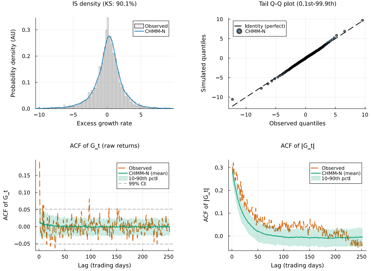
Figure 10. IS SPY CHMM-N comparison at K = 3 (Pipeline A, 1,000 simulated paths; panels as in Figure 4). The K = 18 counterpart is Figure 4 of the main text.
