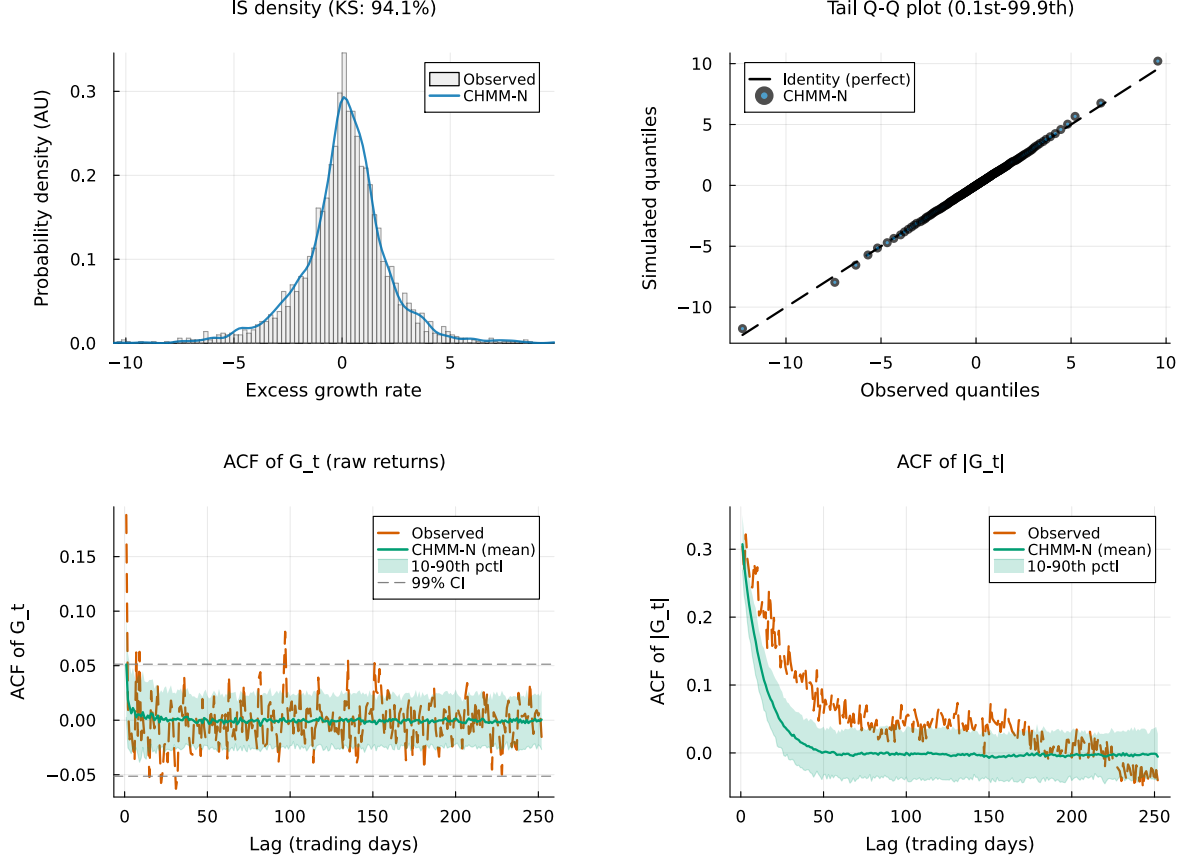
Figure 4. IS CHMM-N validation on SPY ( K = 18 , 1,000 simulated paths). Panel (a): marginal density of the annualized excess log return G_t ; gray histogram = observed IS series, blue curve = one simulated path. Panel (b): tail Q-Q plot at 200 quantile levels; blue points = simulated pooled over paths, black dashed = identity. Panel (c): ACF of raw G_t at lags 1–252 (linear autocorrelation); orange dashed = observed, green = mean across sim paths, shaded band = 10th–90th percentile across sim paths, dashed grey = 99% Bartlett confidence band. Panel (d): ACF of |G_t| on the same window (volatility clustering); same colour conventions. The 2x2 layout mirrors the empirical-only Figure 3: panels (a/b) verify marginal fidelity, panels (c/d) the two ACF-based stylized facts.
