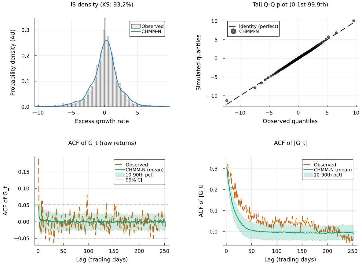
Figure 12. IS SPY CHMM-N comparison at K = 12 (Pipeline A, 1,000 simulated paths; panels as in Figure 4).
