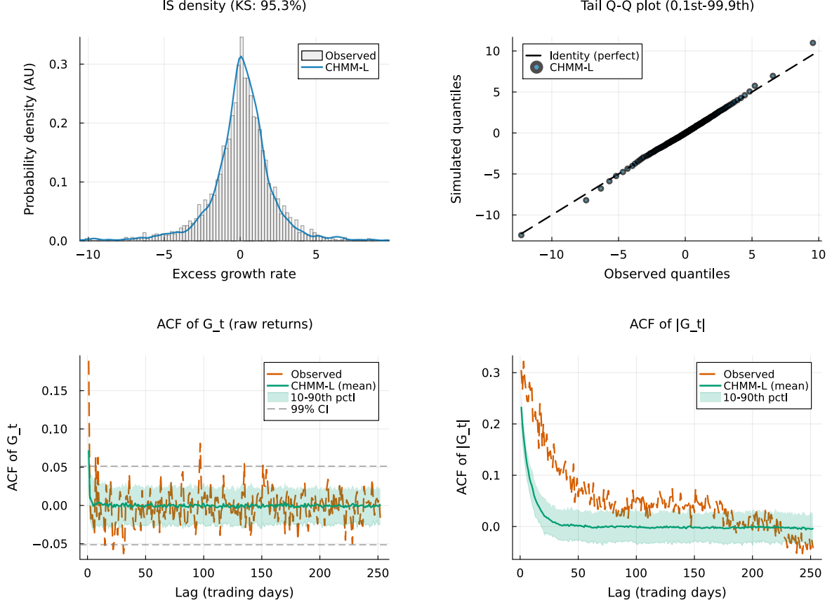
Figure 21. IS SPY model comparison at K = 18 for CHMM-L Laplace emissions (Pipeline A, 1,000 simulated paths). Panels as in Figure 20.
