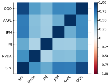
(b) Single Index Model.
