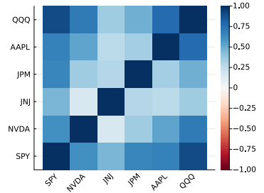
(c) Gaussian copula.
