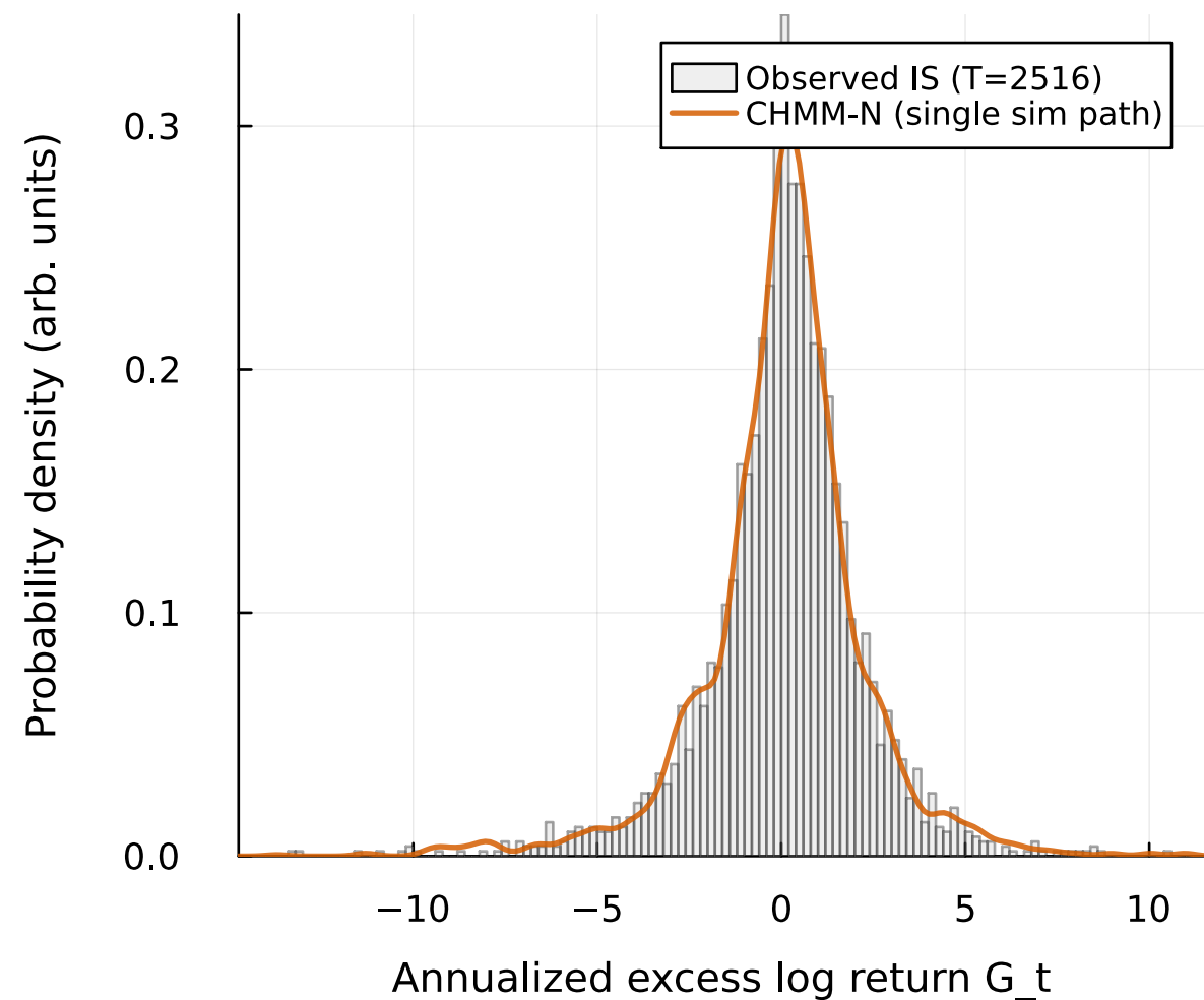
(a) IS return density | KS pass rate = 93.9% of 1000 paths at alpha=0.05
