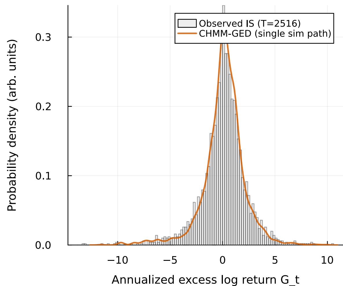
(a) IS return density | KS pass rate = 96.3% of 1000 paths at alpha=0.05
