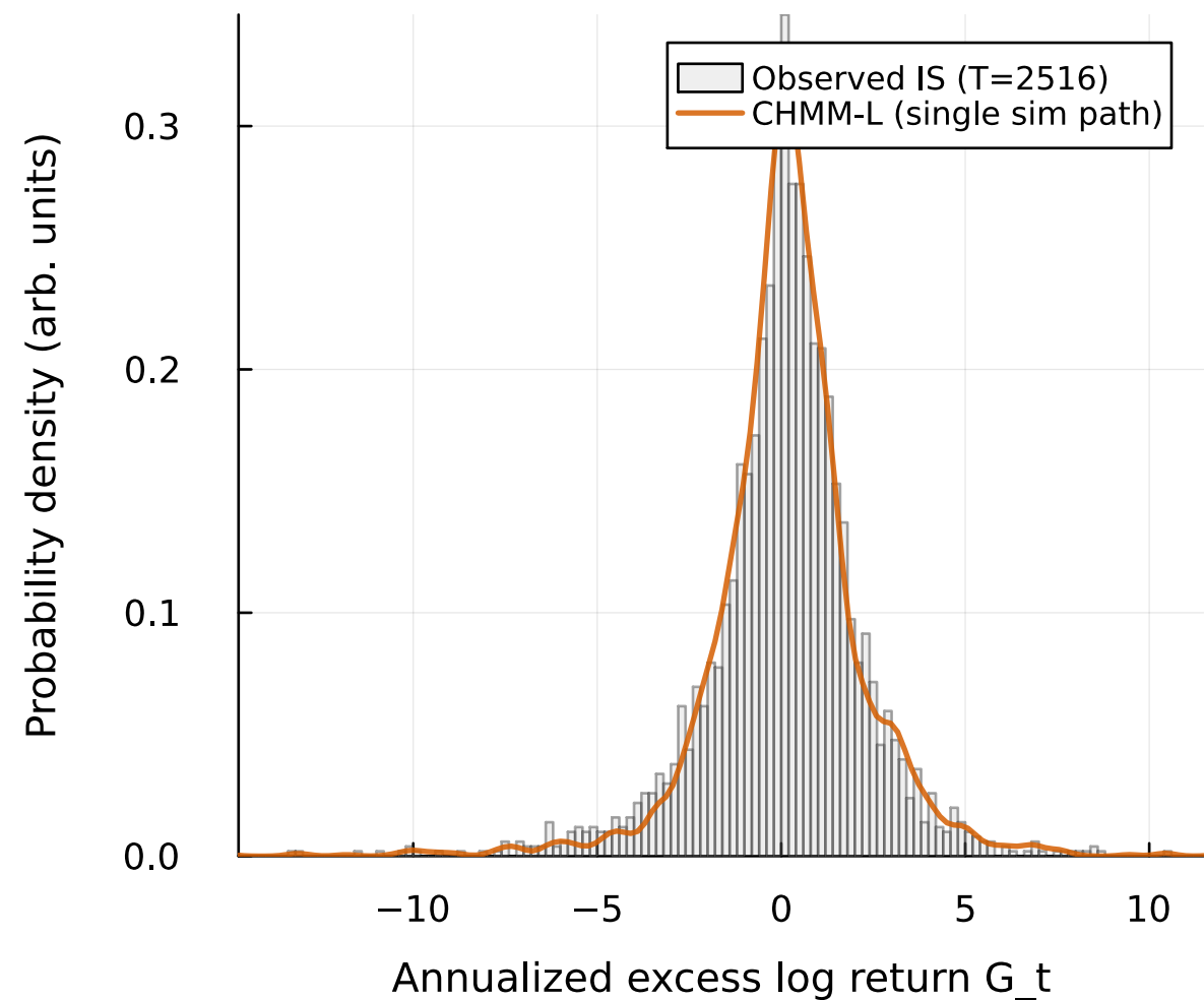
(a) IS return density | KS pass rate = 94.2% of 1000 paths at alpha=0.05
