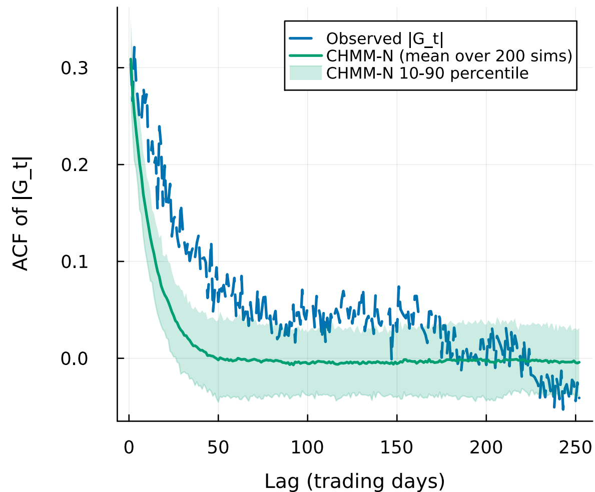
(b) ACF of |G_t| | lag 1..252 (trading days)
