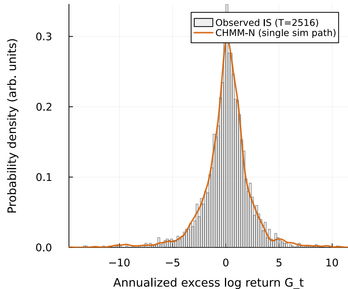
(a) IS return density | KS pass rate = 95.3% of 1000 paths at alpha=0.05
