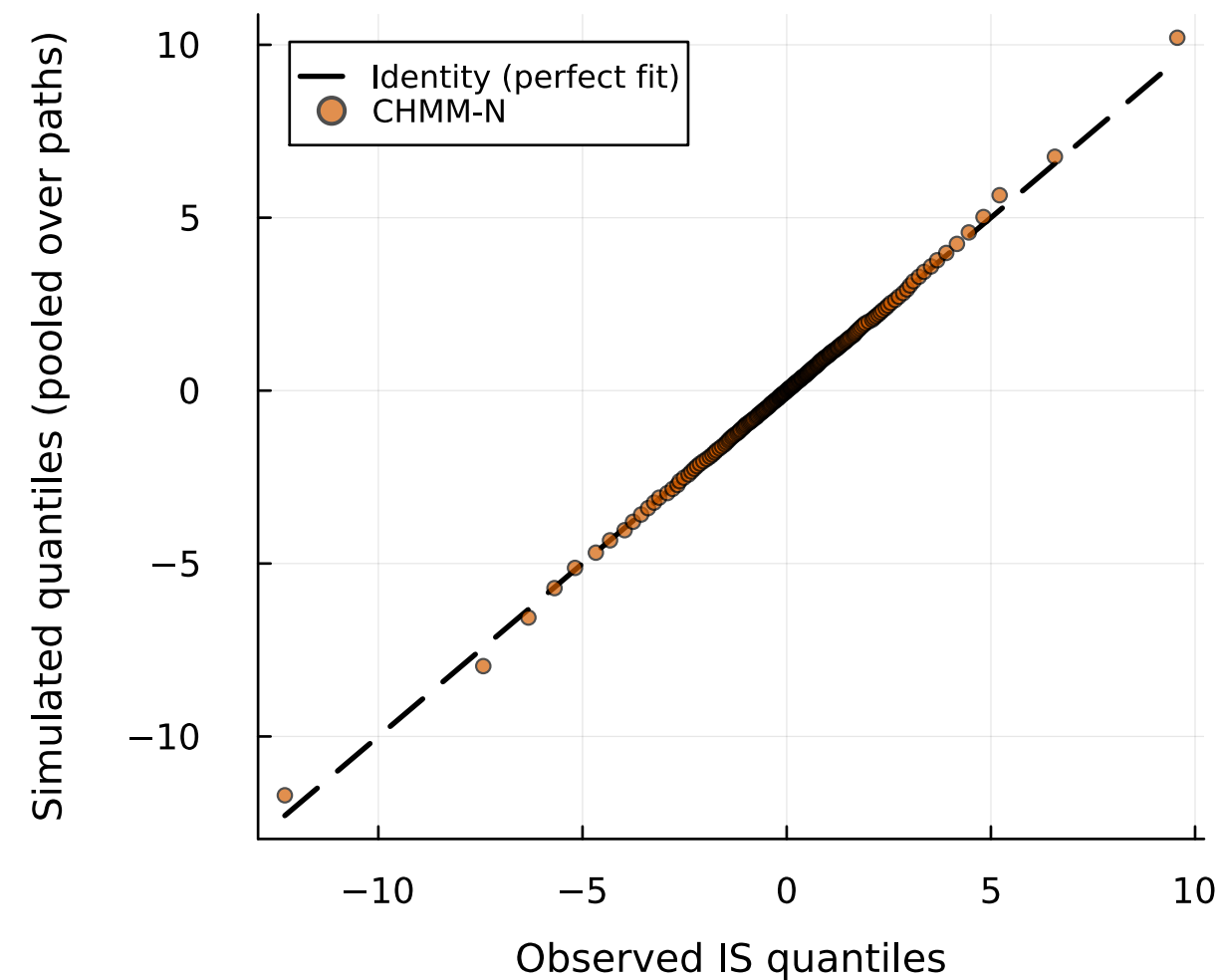
(c) Tail Q-Q plot | quantile grid 0.1% .. 99.9%
