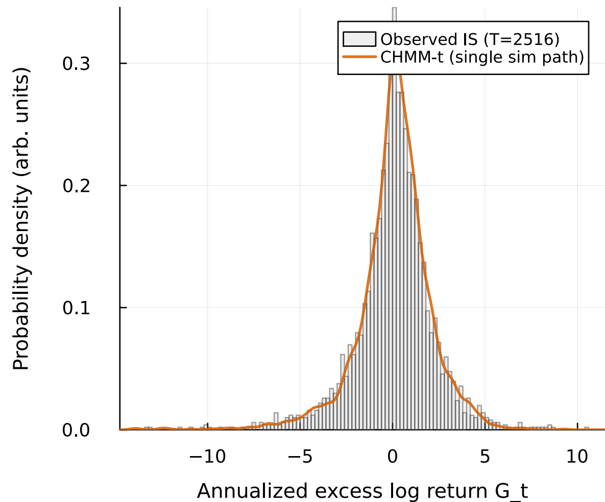
(a) IS return density | KS pass rate = 94.6% of 1000 paths at alpha=0.05
