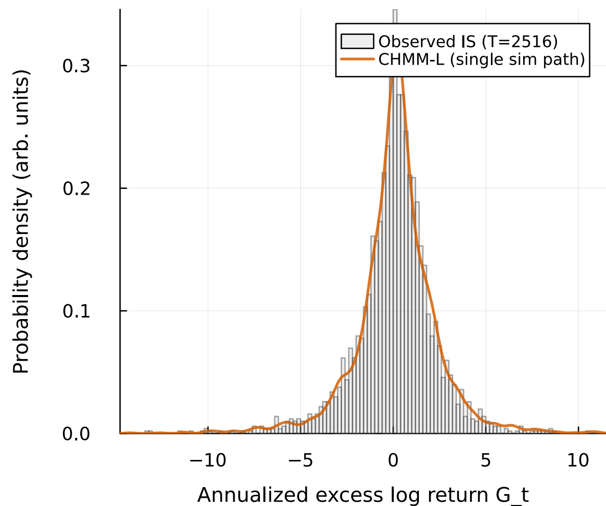
(a) IS return density | KS pass rate = 80.5% of 1000 paths at alpha=0.05
