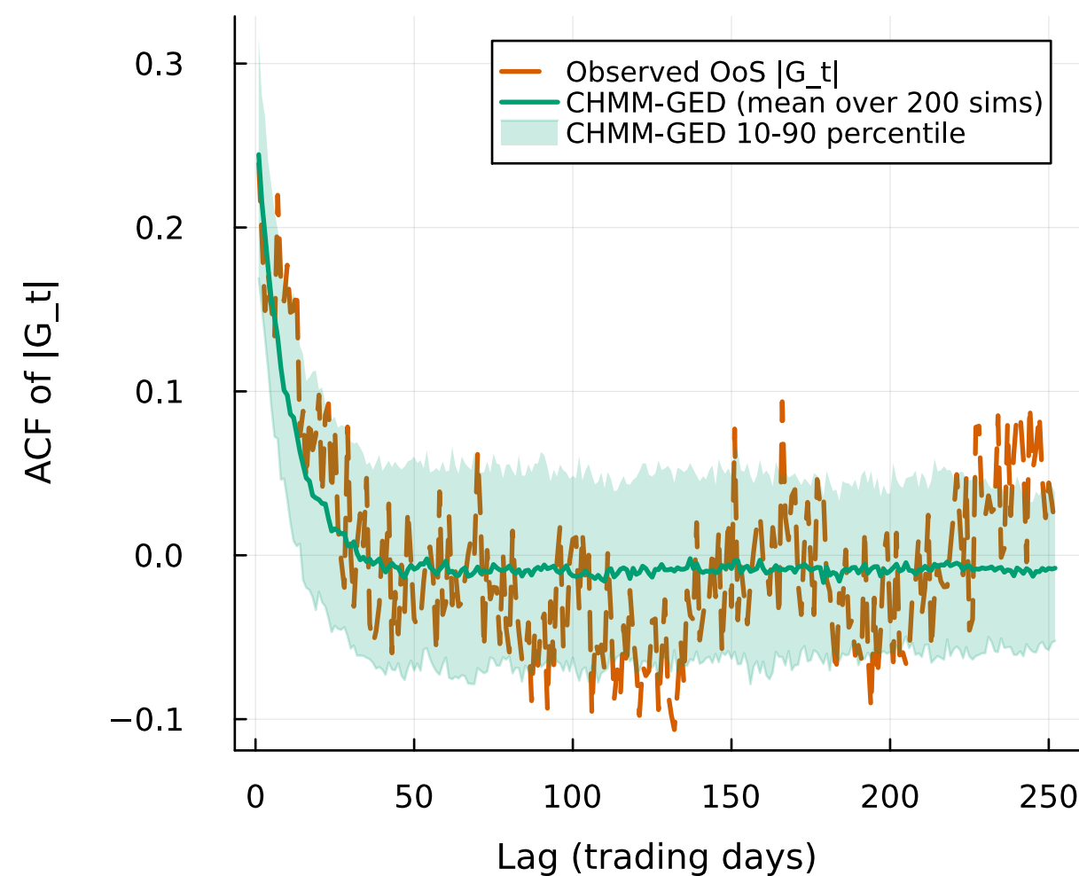
(c) OoS ACF of |G_t| | lag 1..252 (trading days)
