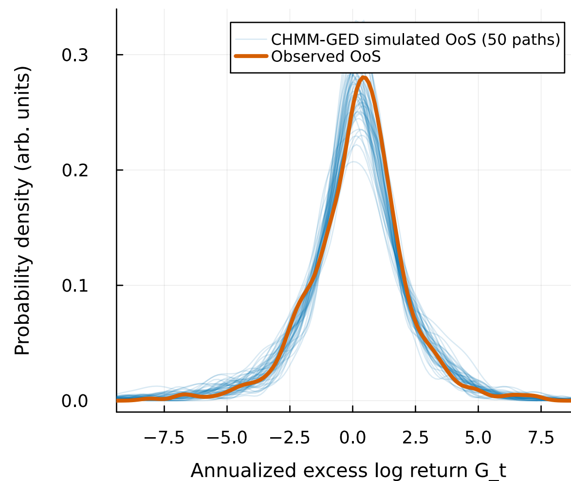
(b) OoS return density fan | 50 sim paths vs. observed OoS (T=572)
