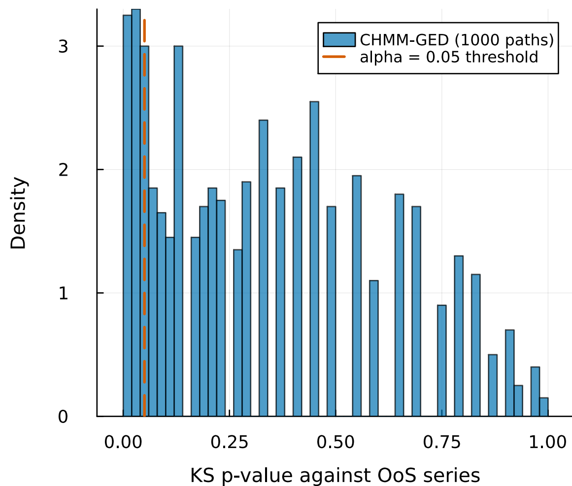
(a) OoS KS p-values | pass rate = 83.8% above alpha=0.05
