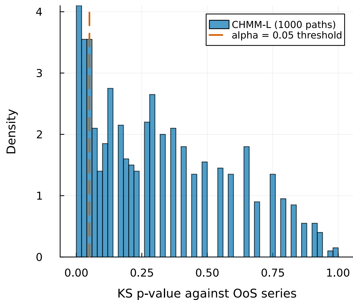
(a) OoS KS p-values | pass rate = 80.5% above alpha=0.05
