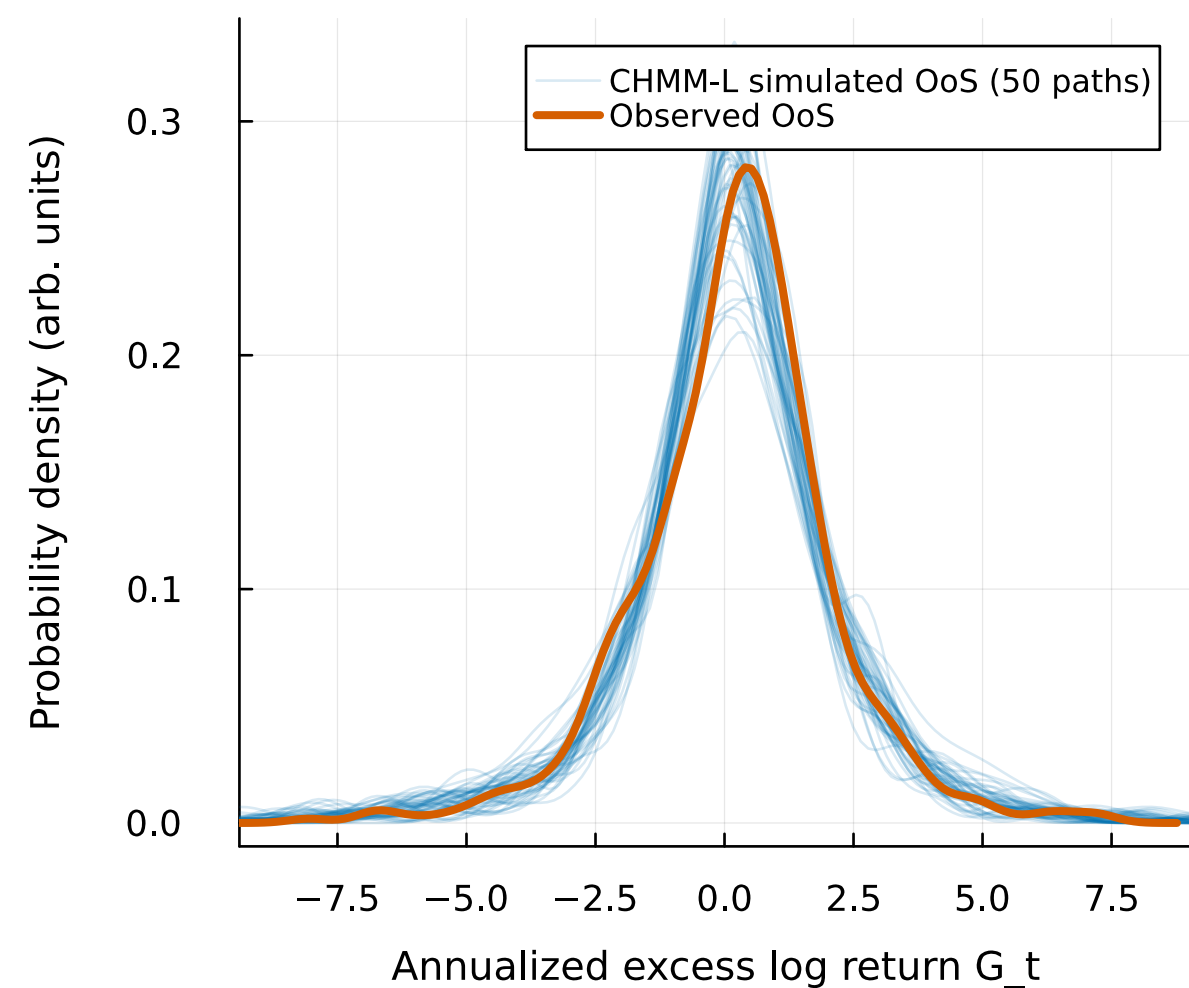
(b) OoS return density fan | 50 sim paths vs. observed OoS (T=572)
