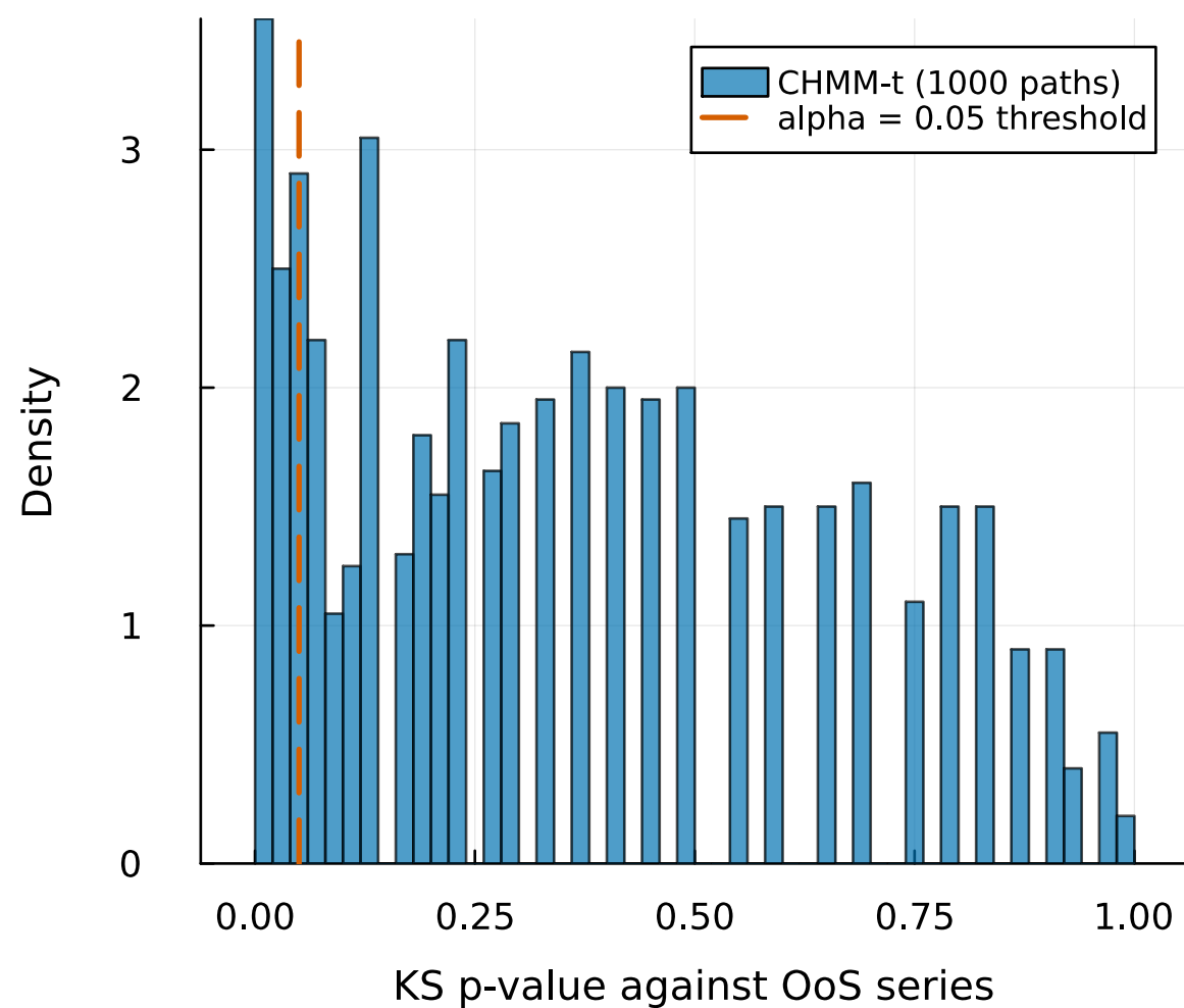
(a) OoS KS p-values | pass rate = 85.0% above alpha=0.05
