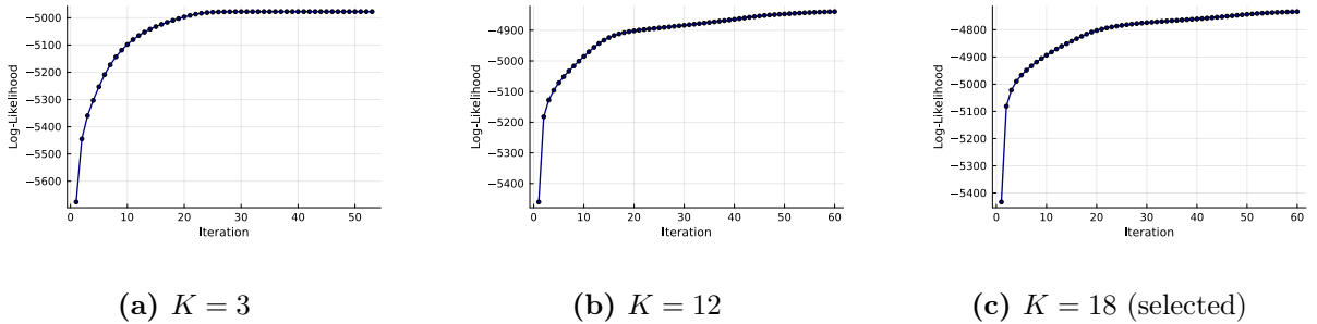
Figure 9. Baum-Welch convergence for the SPY CHMM-N fit (Pipeline A, IS) at selected state resolutions. Log-likelihood is monotonically increasing (EM guarantee) and plateaus well before \text{max\_iter} = 60 .
