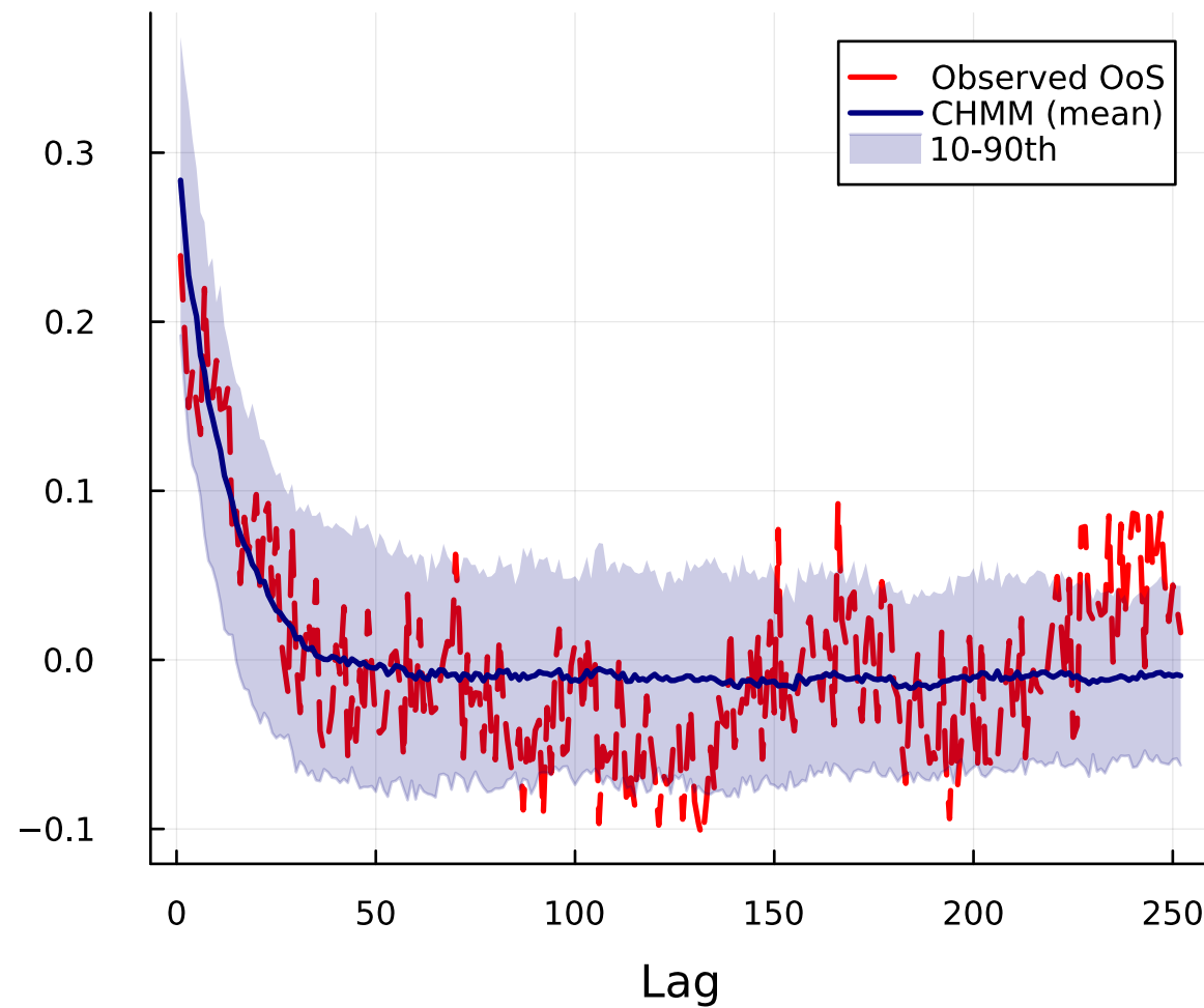
(c) OoS ACF( |G_t| )
