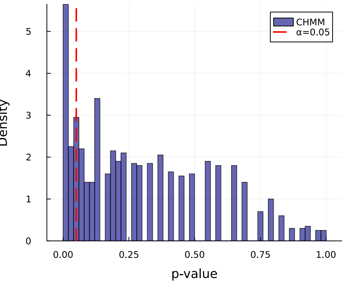
(a) OoS KS p-values
