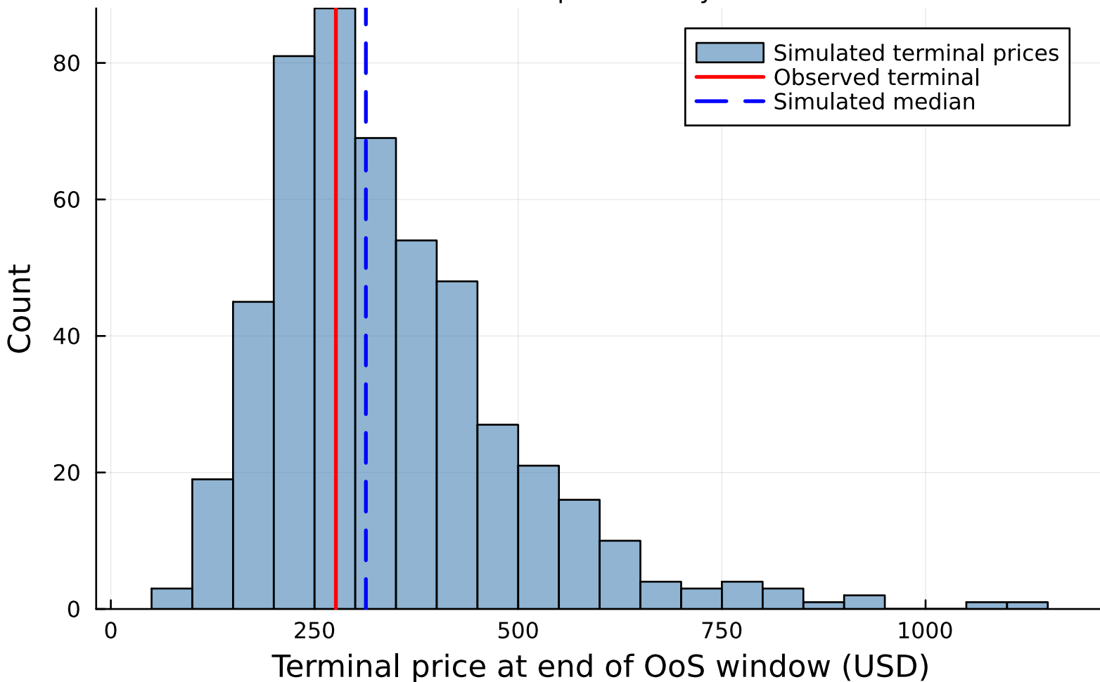
Pipeline A — AAPL terminal-price distribution | CHMM-N, K=18 500 simulated paths at day 572 OoS
