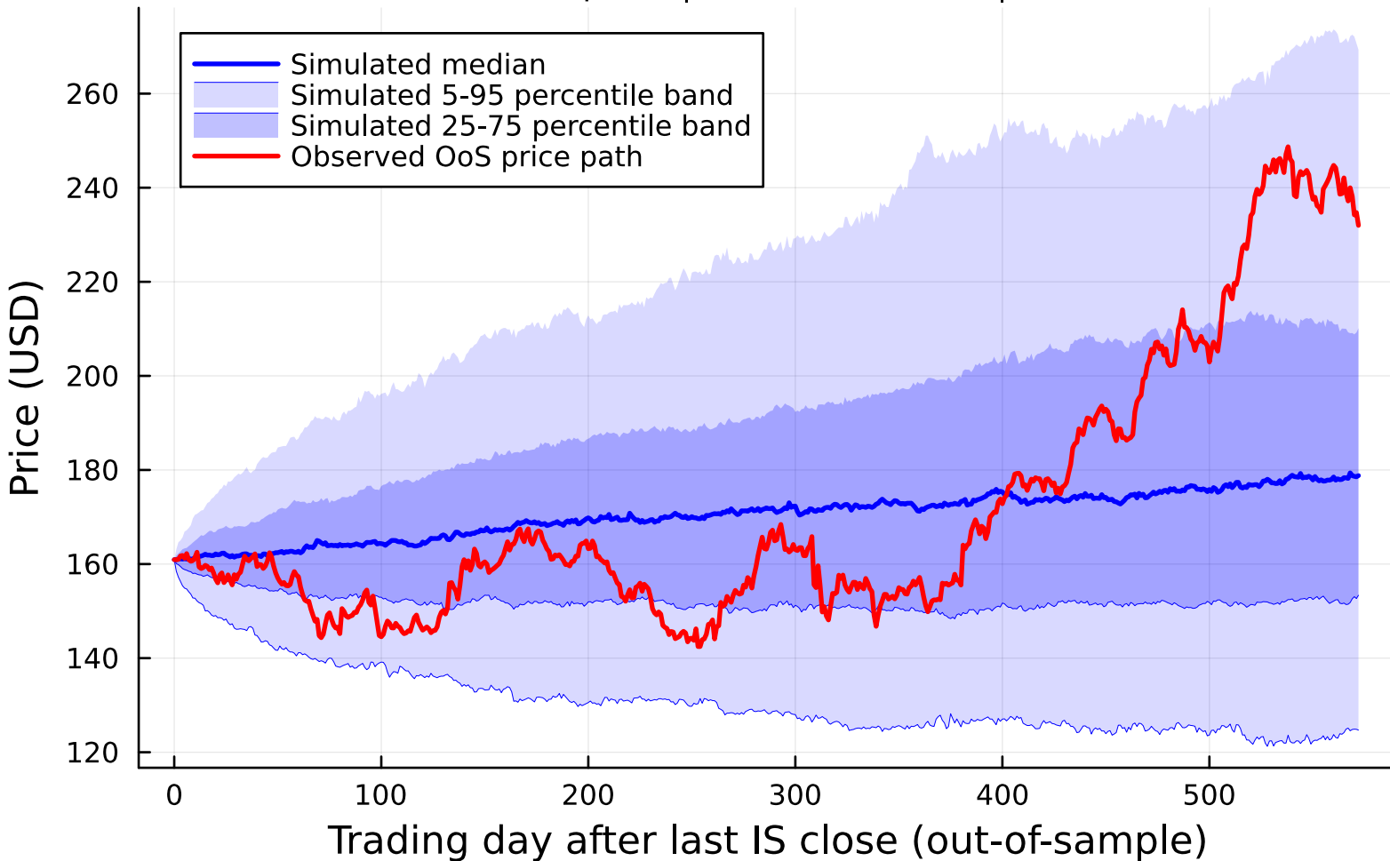
Pipeline A — JNJ OoS price fan | CHMM-L, K=18 500 simulated paths | S0 = last IS VWAP | dt = 1/252
