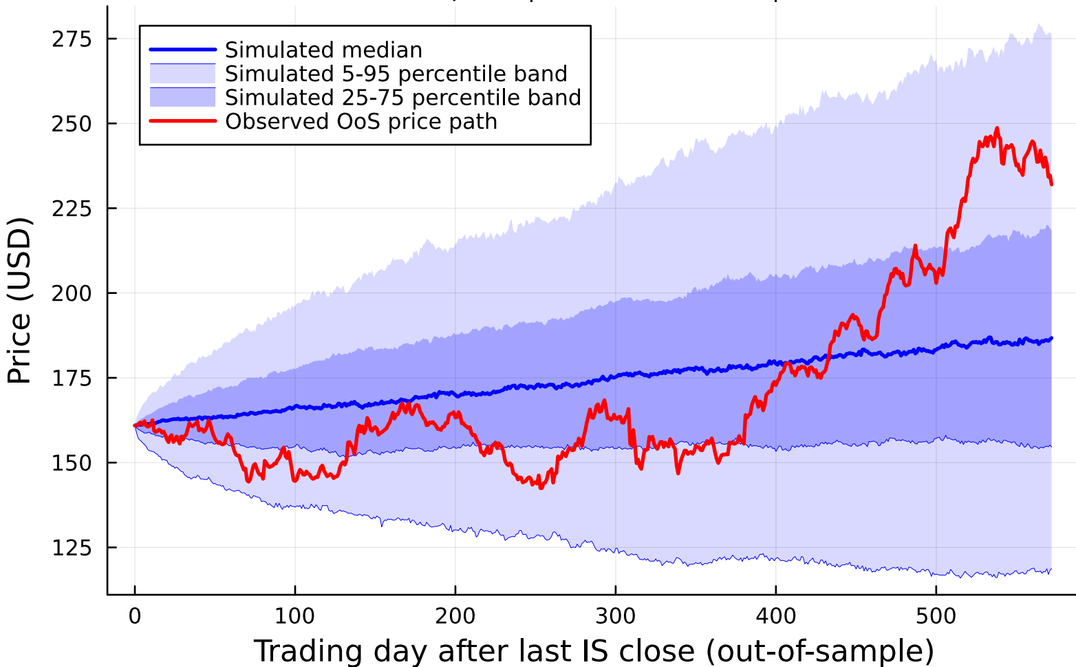
Pipeline A — JNJ OoS price fan | CHMM-N, K=18 500 simulated paths | S0 = last IS VWAP | dt = 1/252
