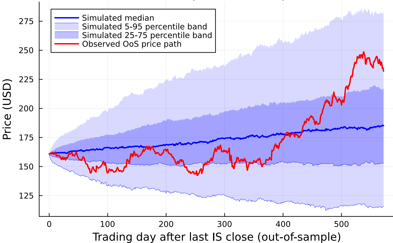
Pipeline A — JNJ OoS price fan | CHMM-t, K=18 500 simulated paths | S0 = last IS VWAP | dt = 1/252
